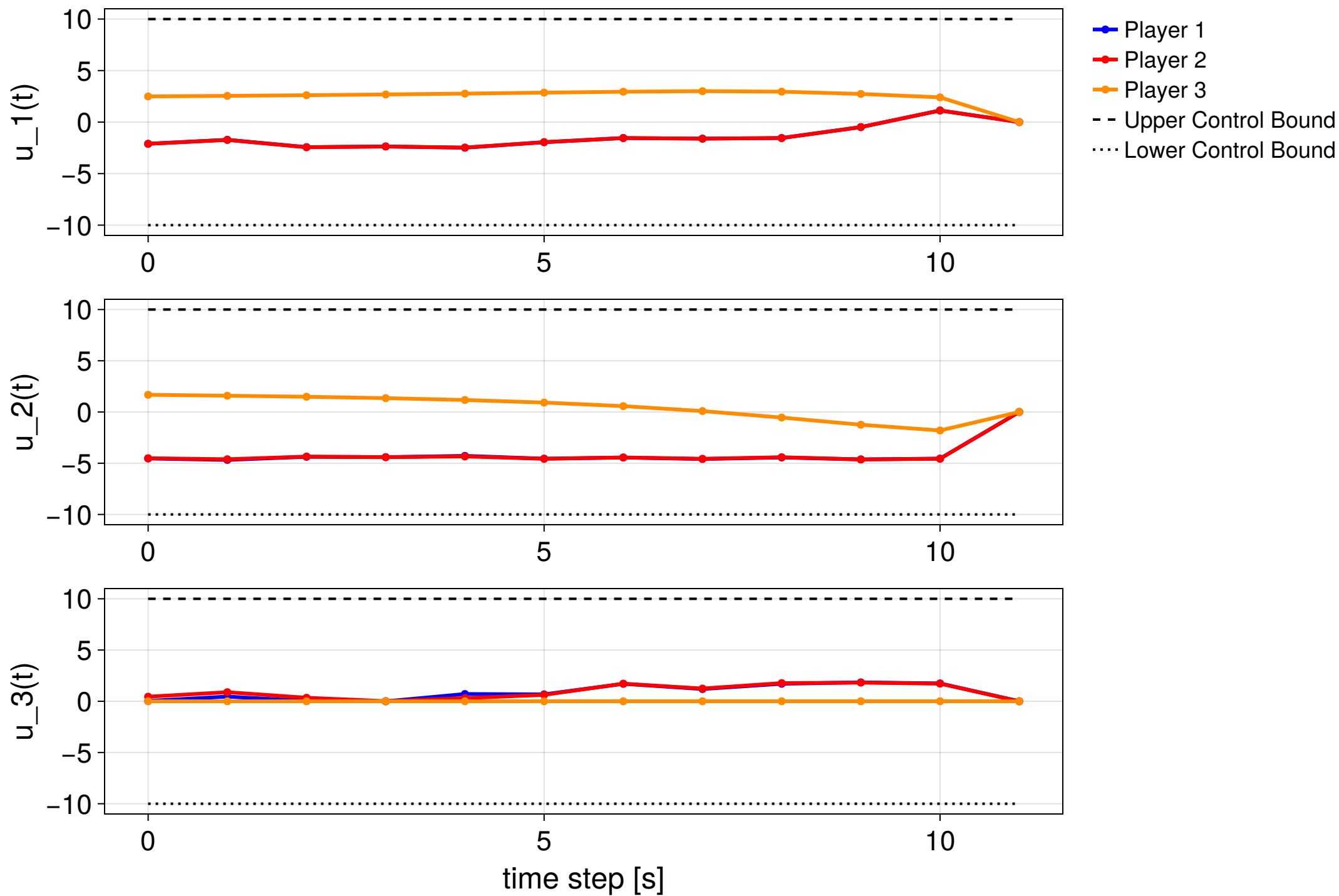
MPC step 4/20 — NOT CONVERGED (KKT error 0.393)
