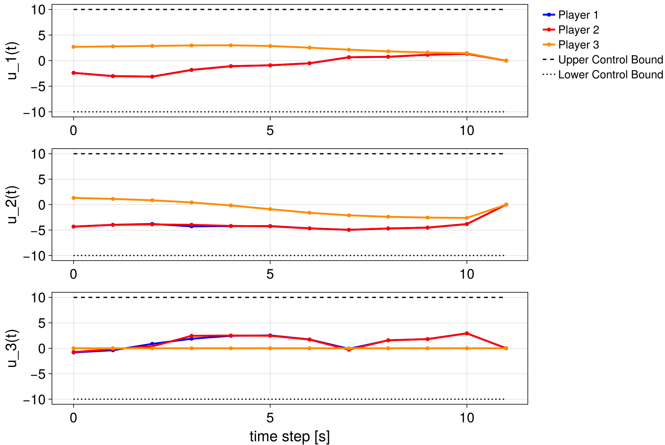
MPC step 7/20 — NOT CONVERGED (KKT error 0.198)
