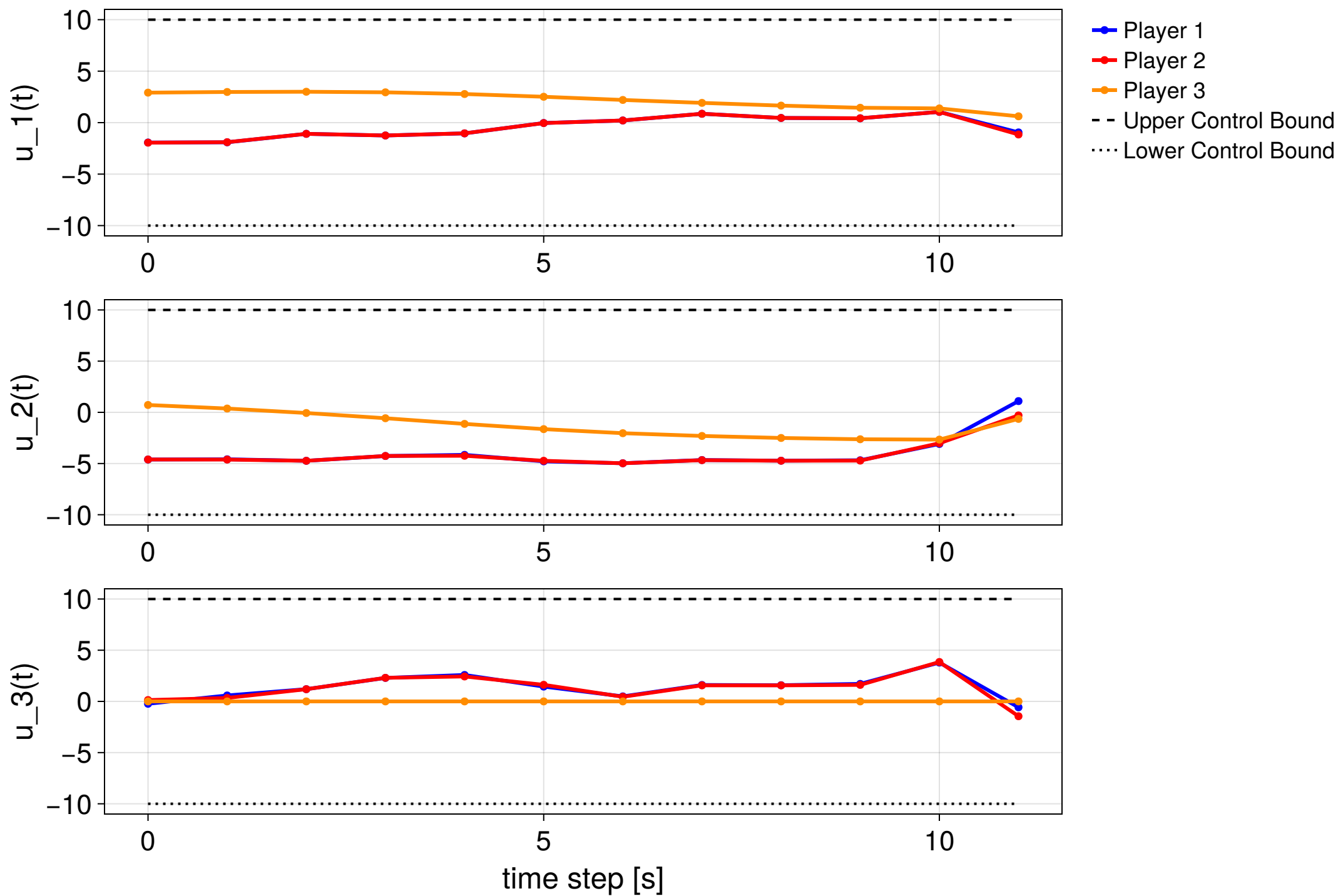
MPC step 8/20 — NOT CONVERGED (KKT error 0.138)
