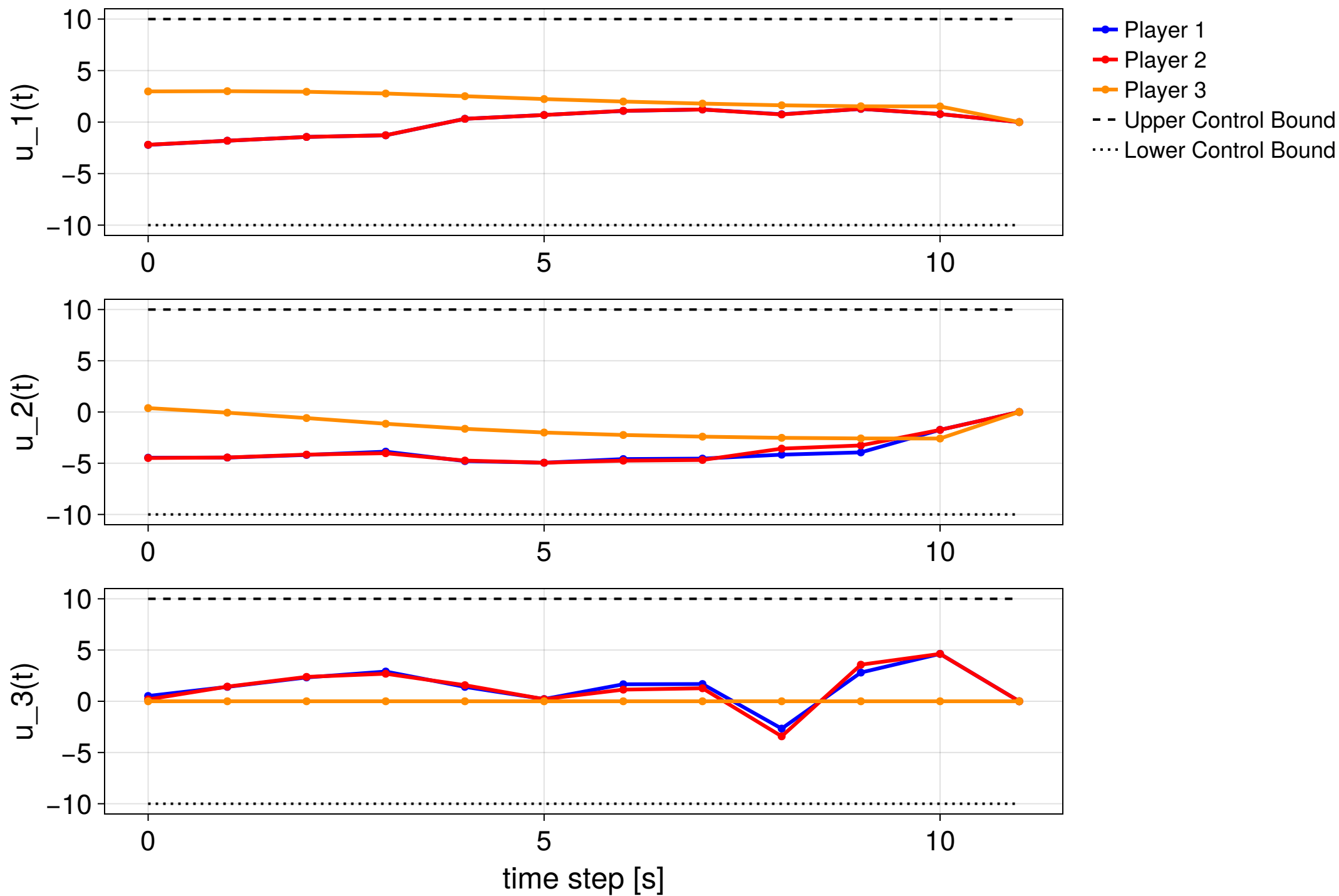
MPC step 9/20 — NOT CONVERGED (KKT error 0.495)
