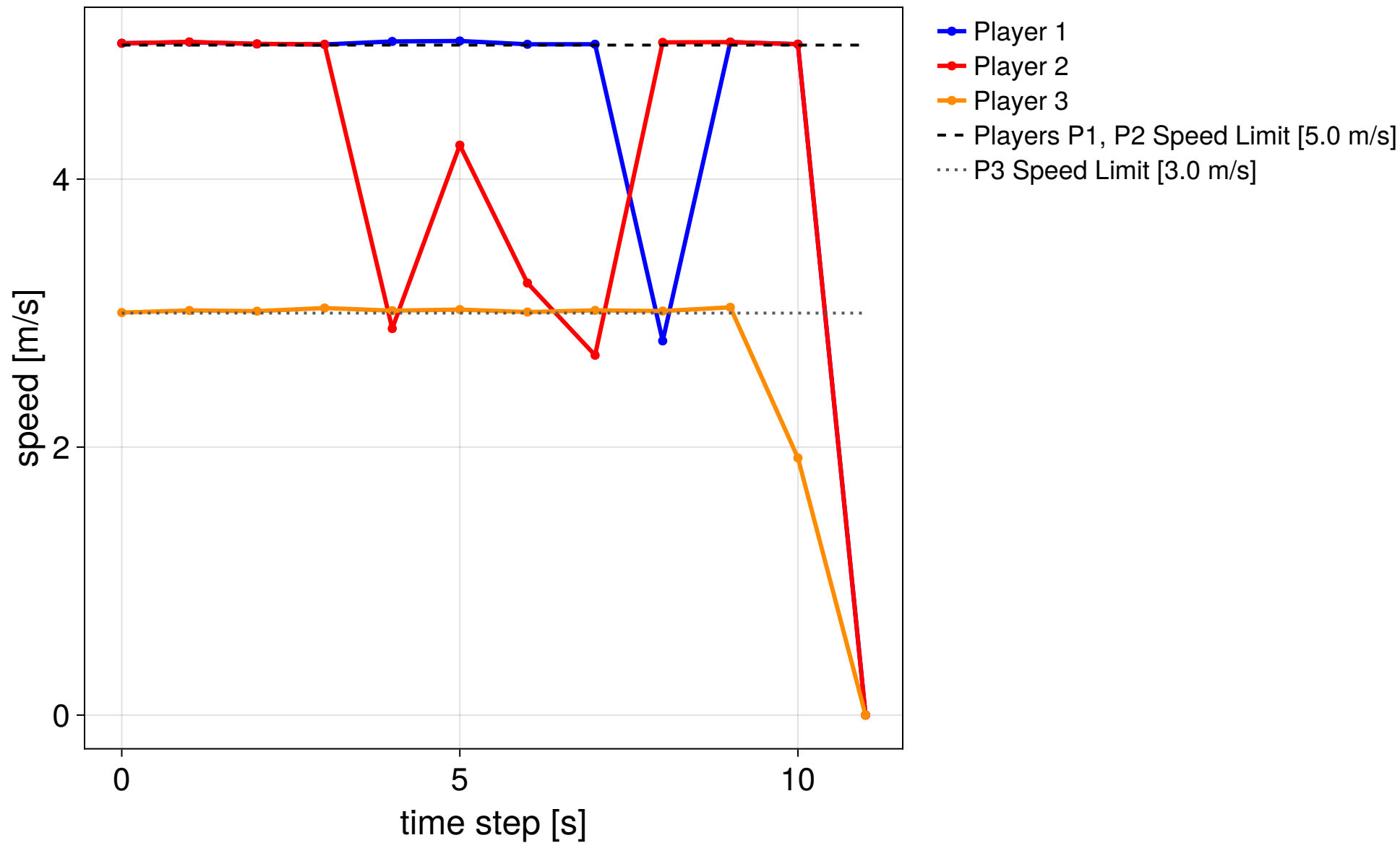
MPC step 16/20 — NOT CONVERGED (KKT error 5.39)
