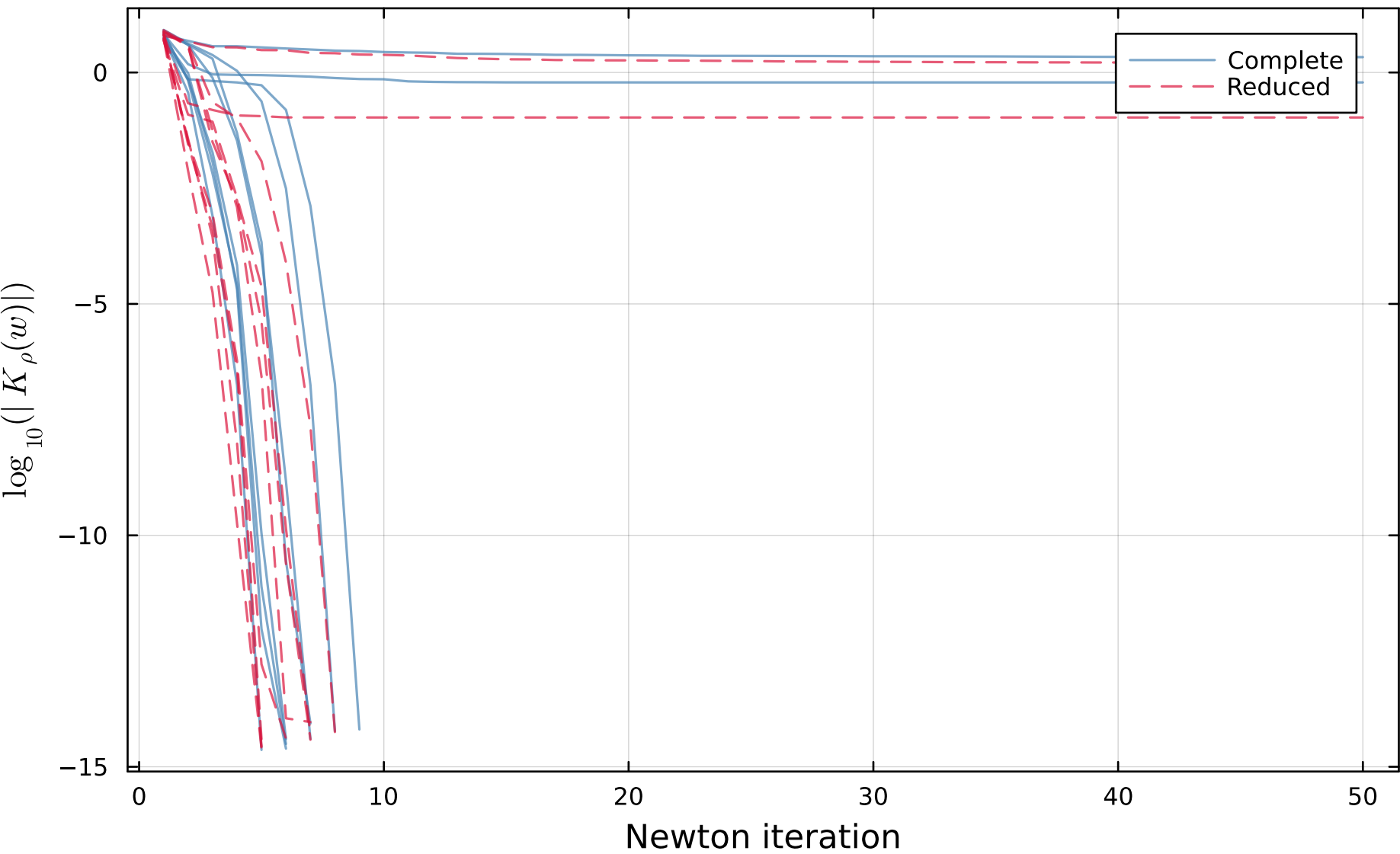
Random QP problems, canonical init ( \rho=0.1 , K=2 , 10 problems)
