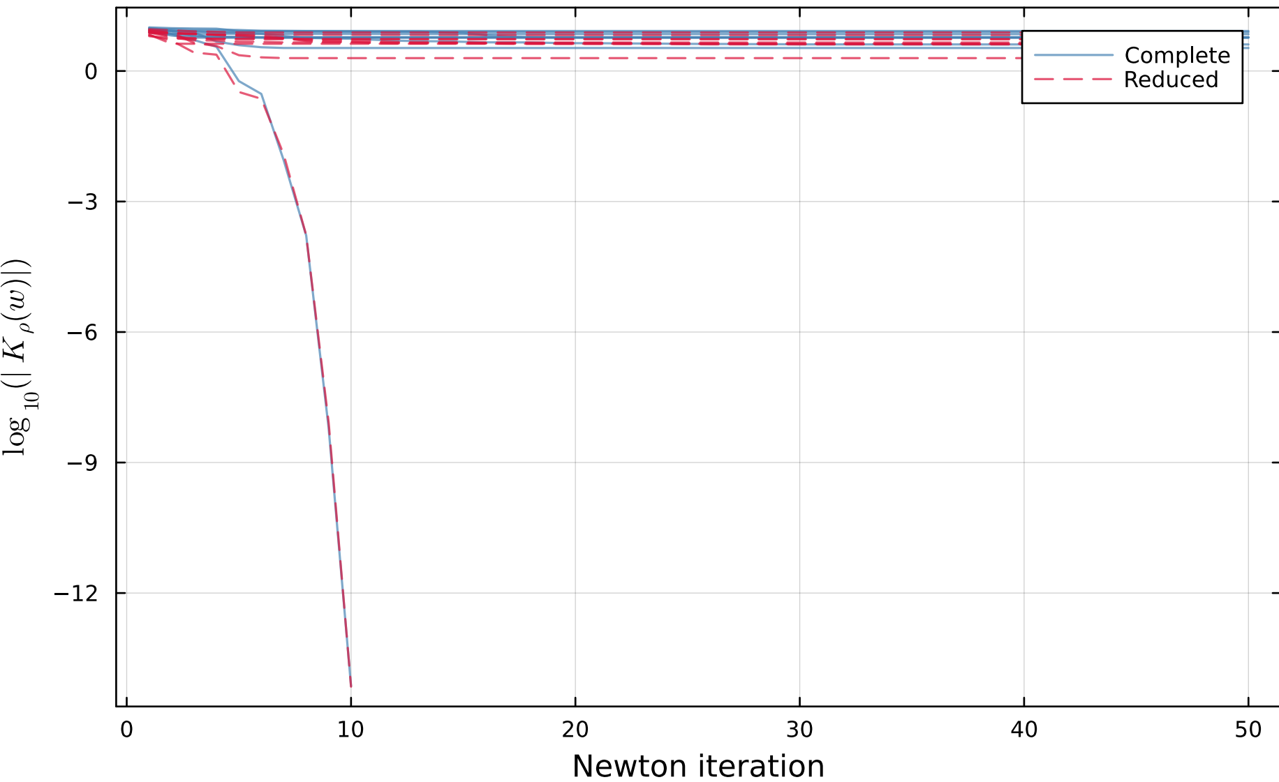
Random QP problems, canonical init ( \rho=1.0 , K=2 , 10 problems)
