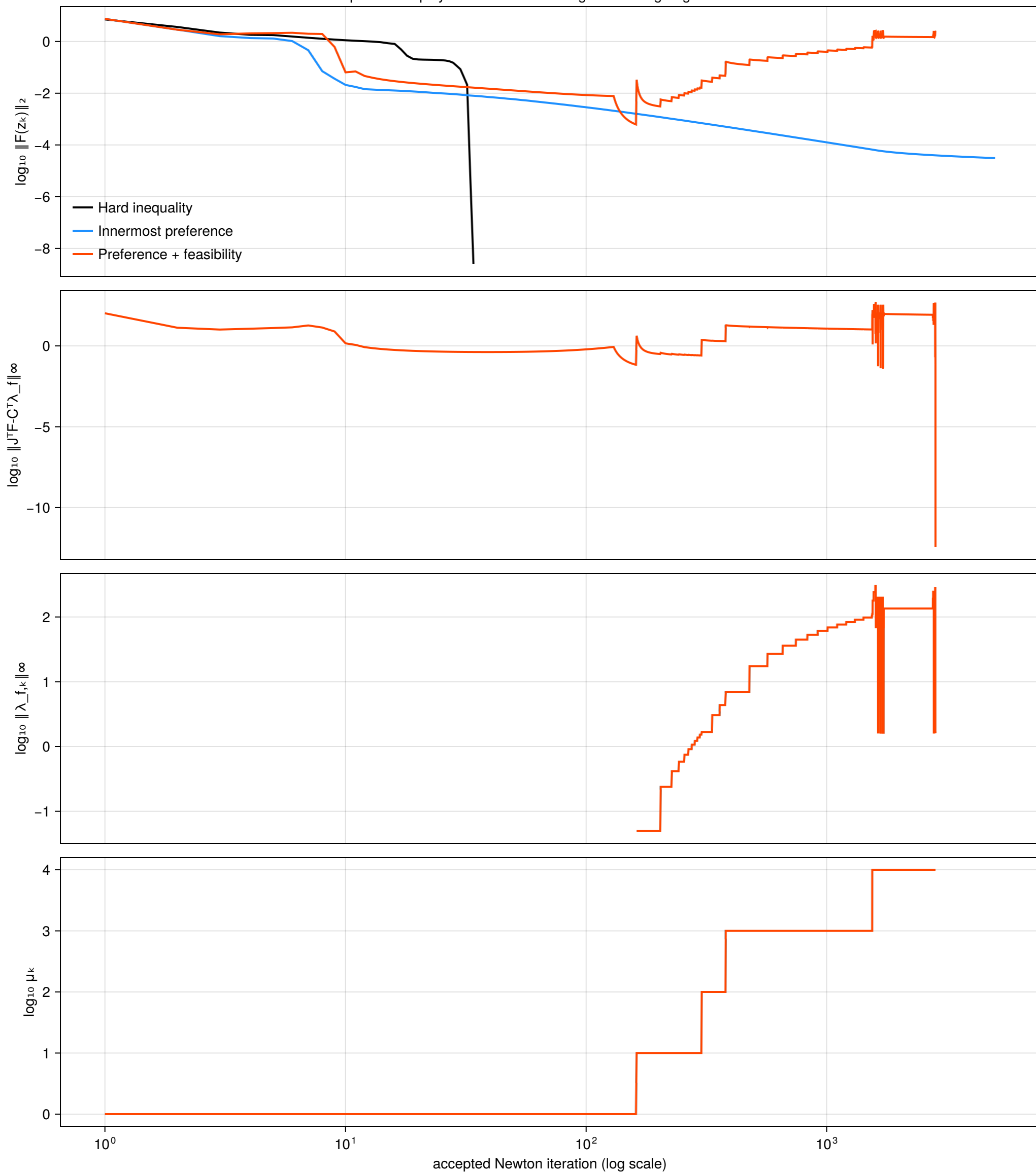
Explicit three-player solve: KKT and augmented-Lagrangian histories
