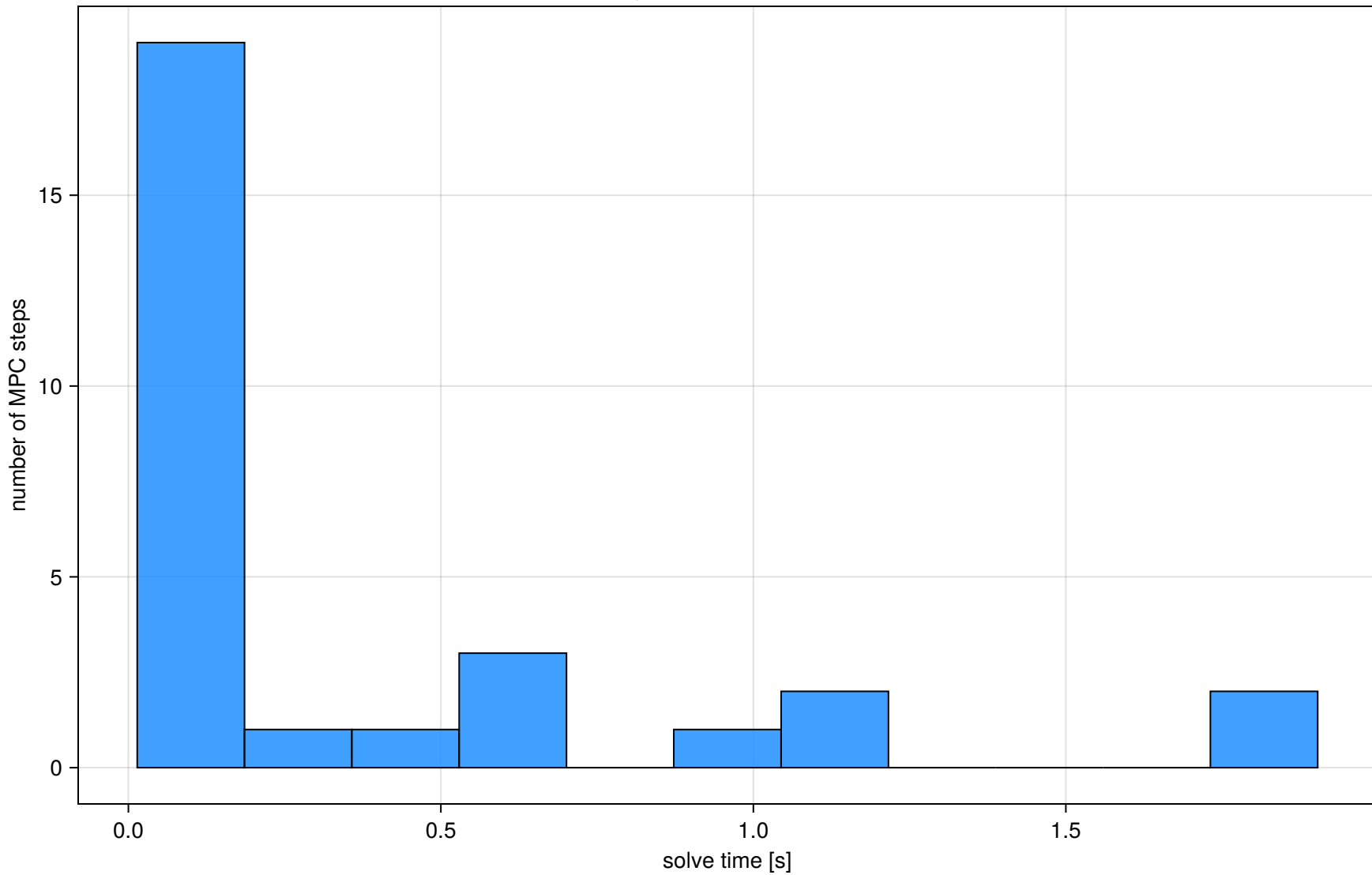
Warm-solve times (step 1 excluded: 1169.0 s incl. one-time JIT)
