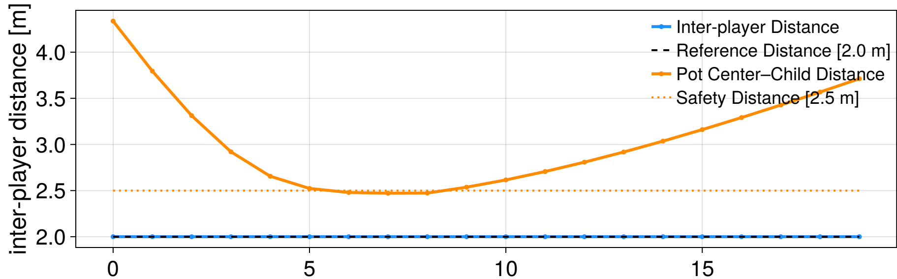
MPC step 6/30
