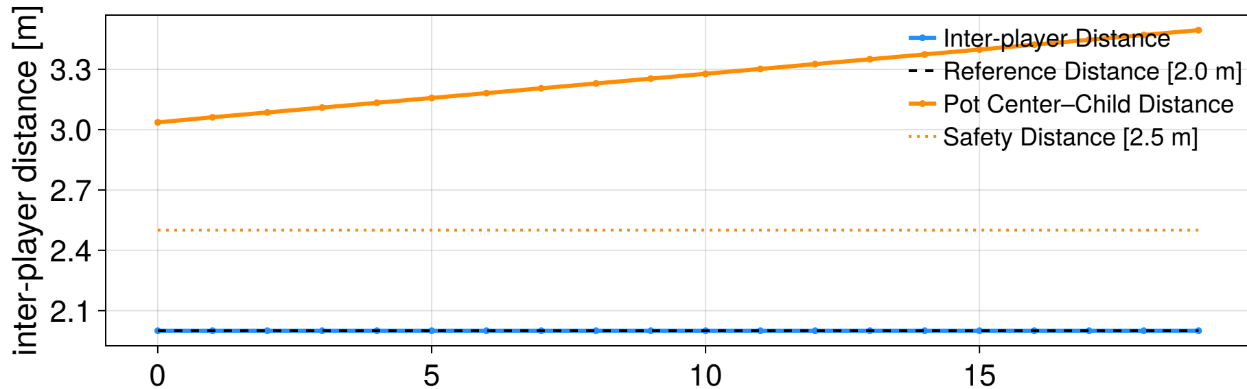
MPC step 29/30
