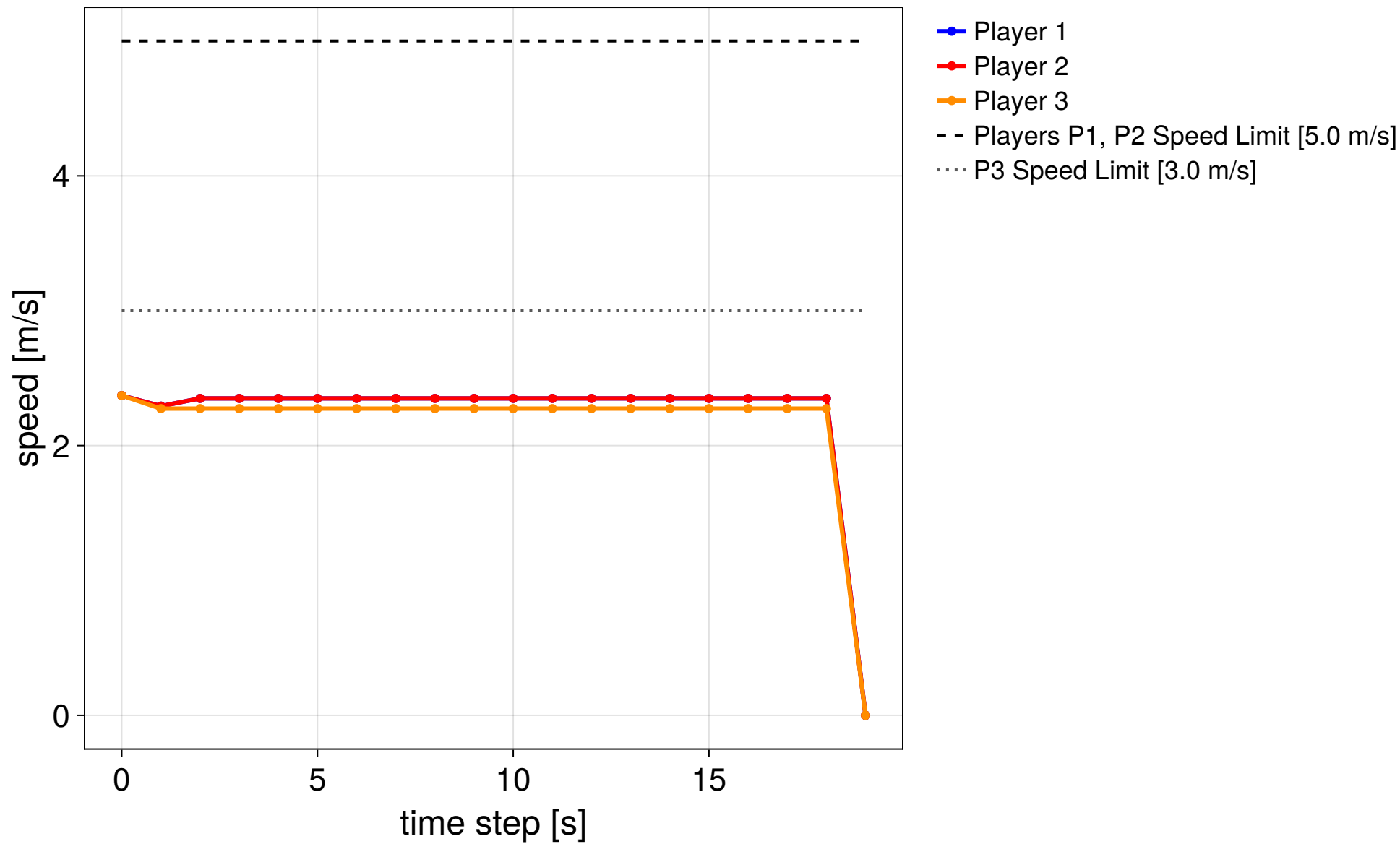
MPC step 21/30
