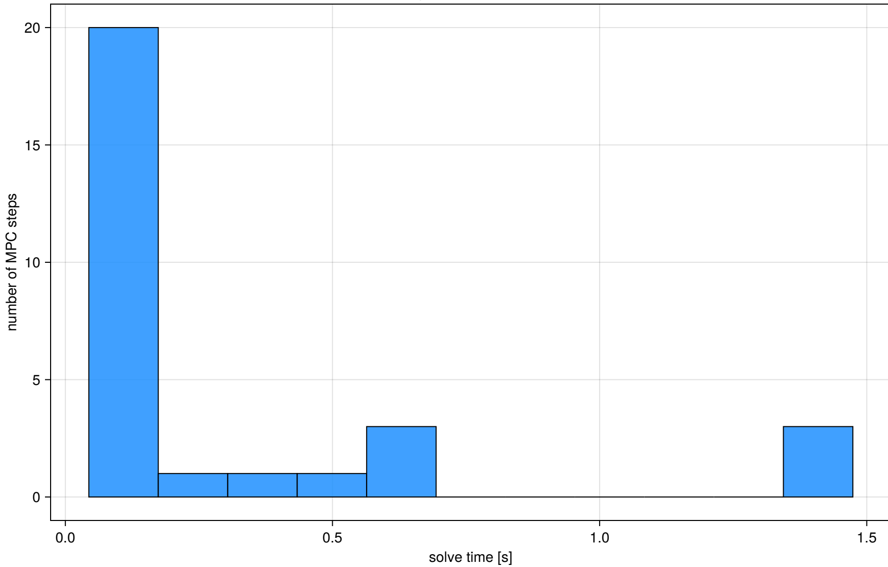
Warm-solve times (step 1 excluded: 65.1 s incl. one-time JIT)
