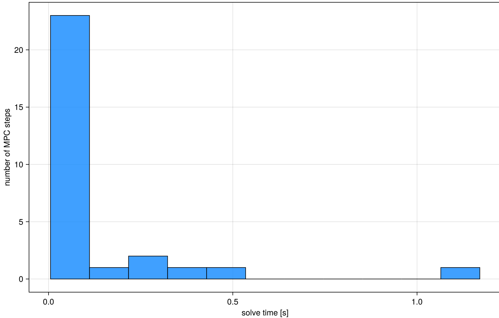
Warm-solve times (step 1 excluded: 61.5 s incl. one-time JIT)
