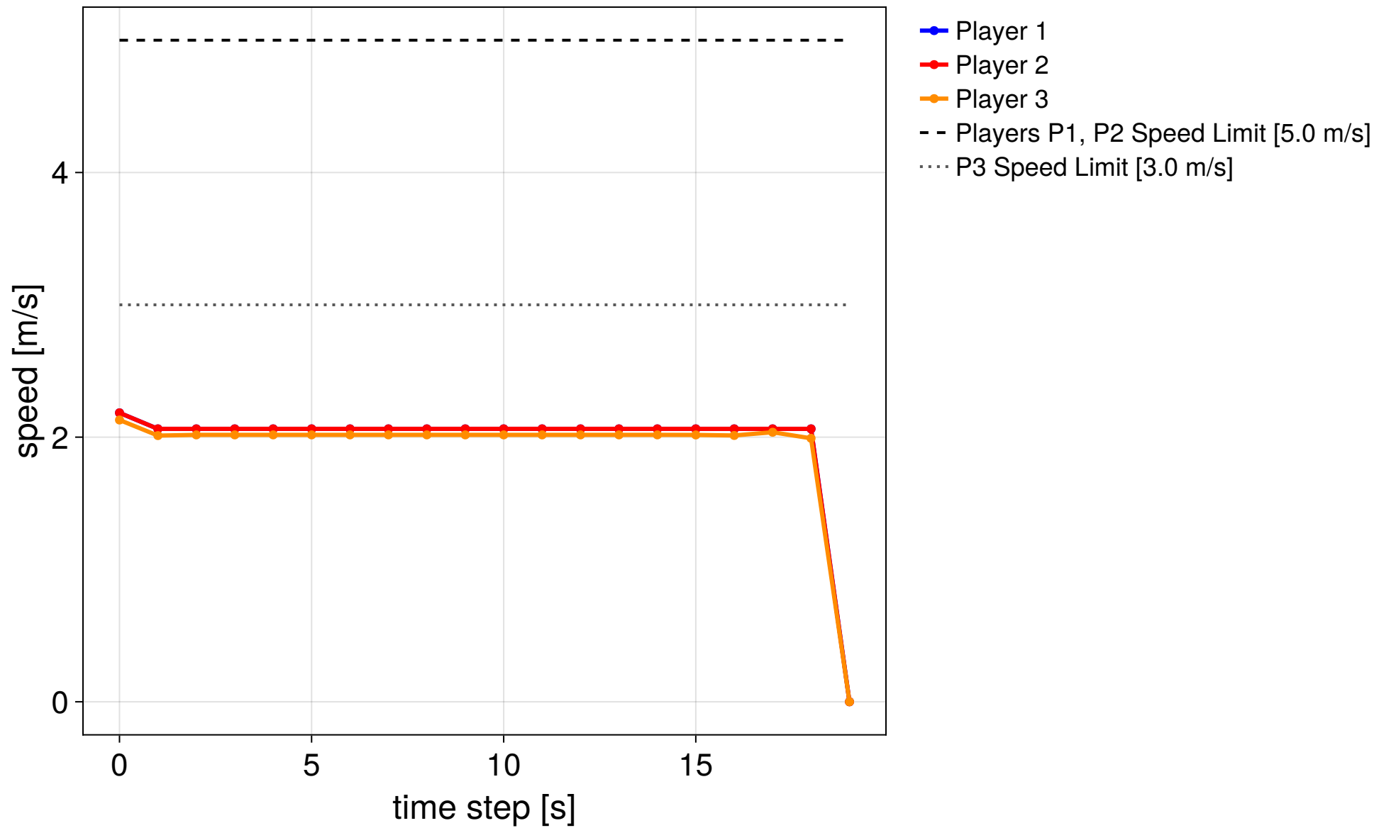
MPC step 20/30
