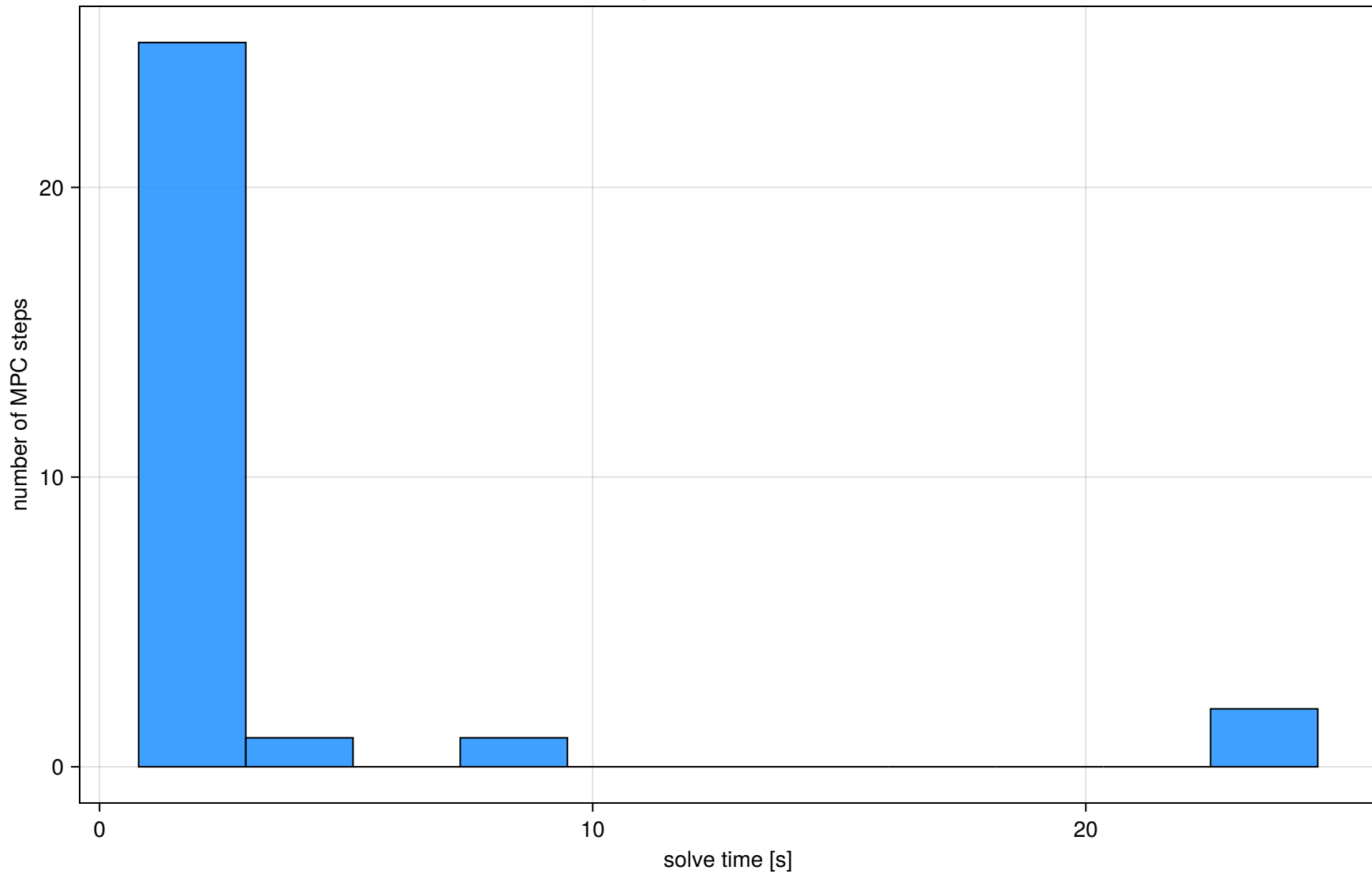
Warm-solve times (step 1 excluded: 351.4 s incl. one-time JIT)
