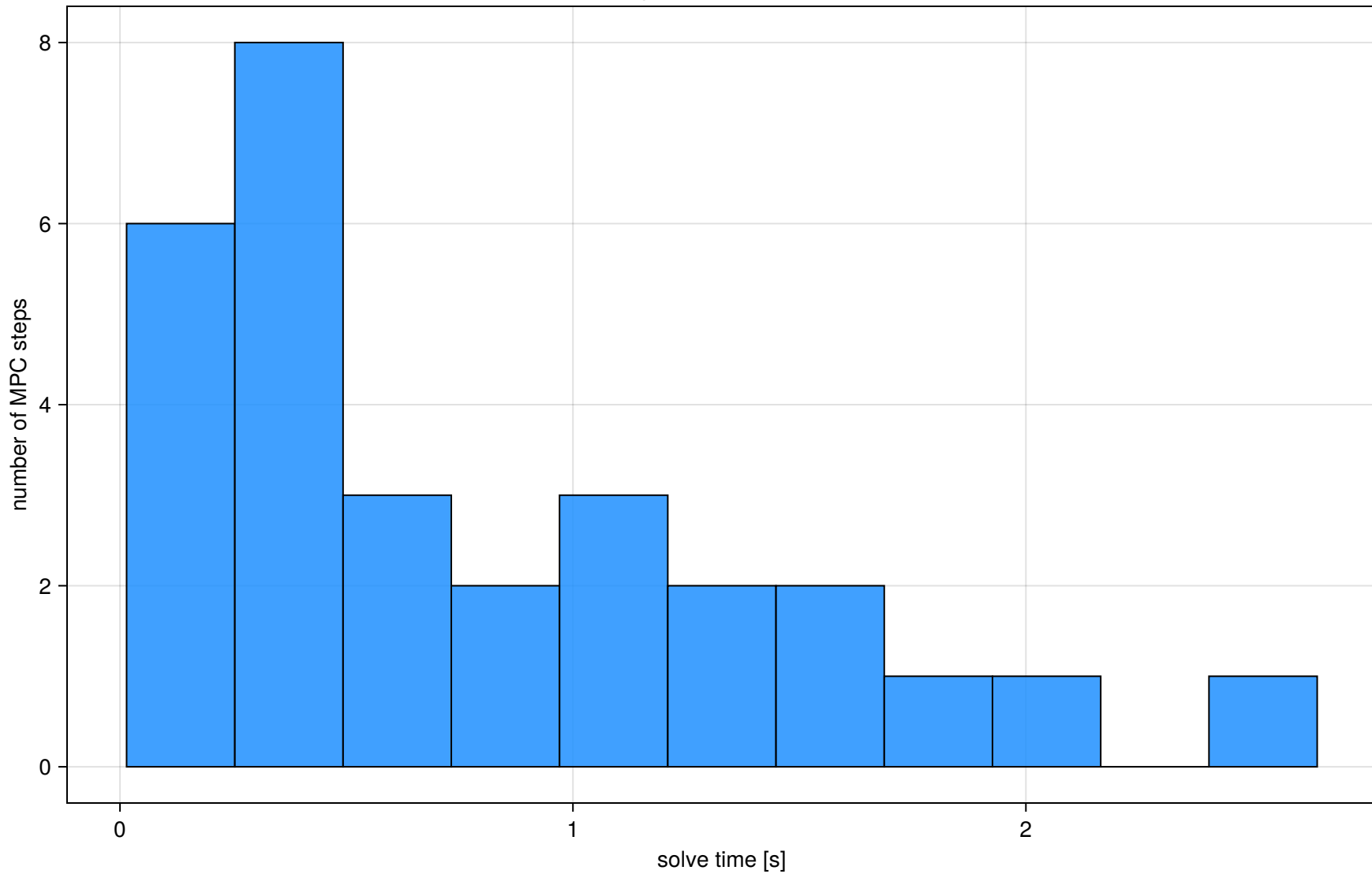
Warm-solve times (step 1 excluded: 66.7 s incl. one-time JIT)
