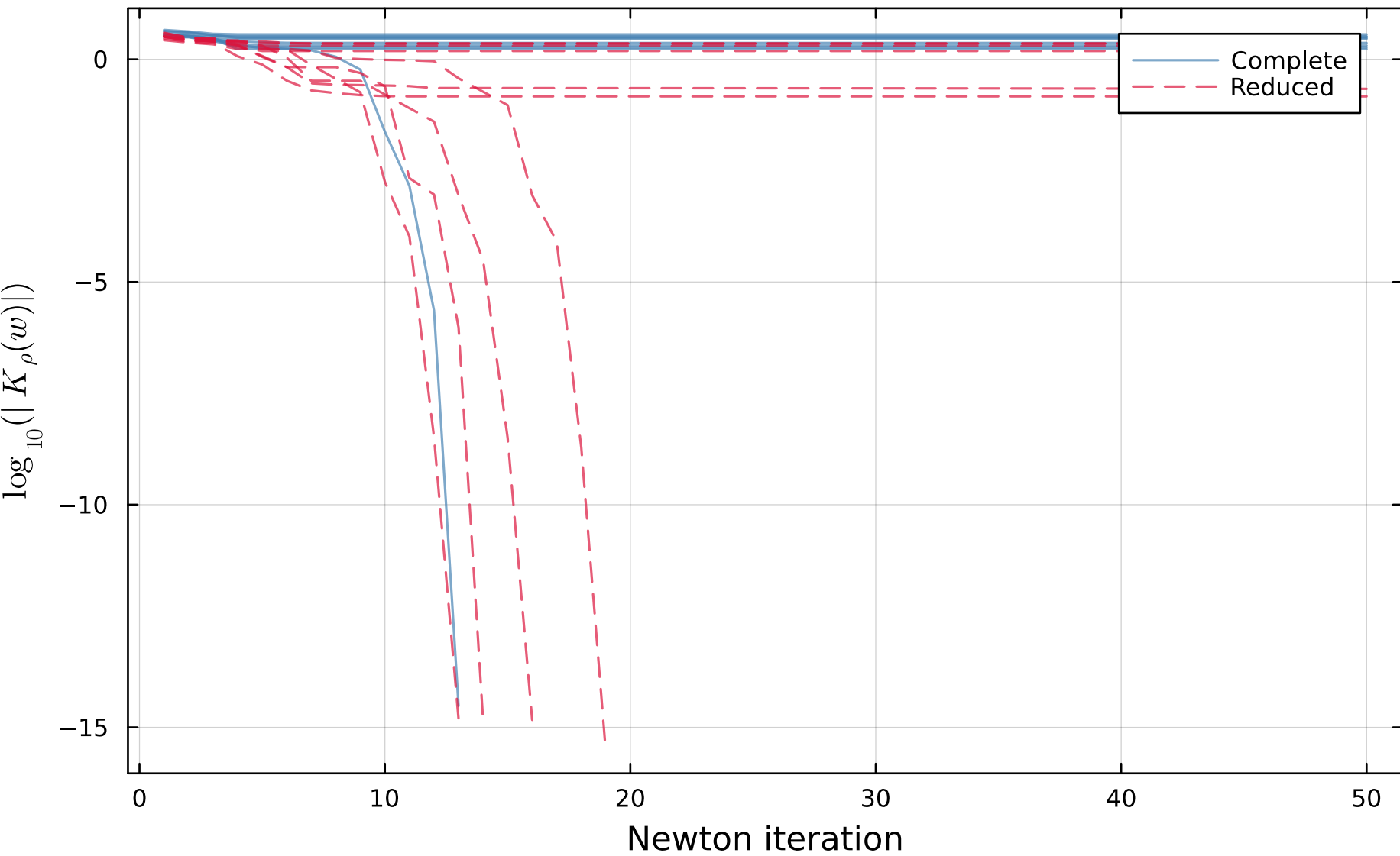
Fixed problem, random init ( \rho=0.001 , K=2 , 10 runs)
