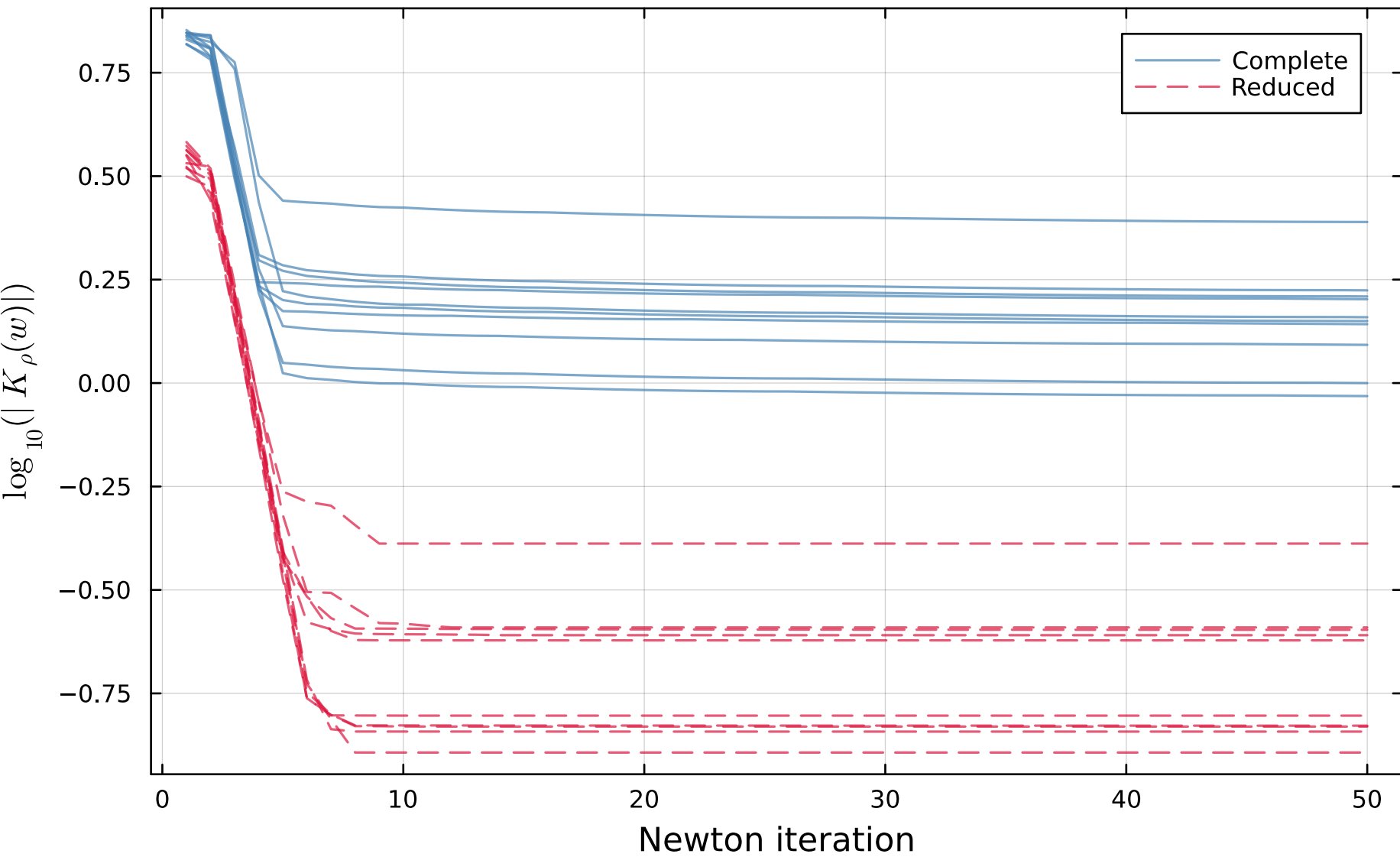
Fixed problem, random init ( \rho=0.001 , K=4 , 10 runs)
