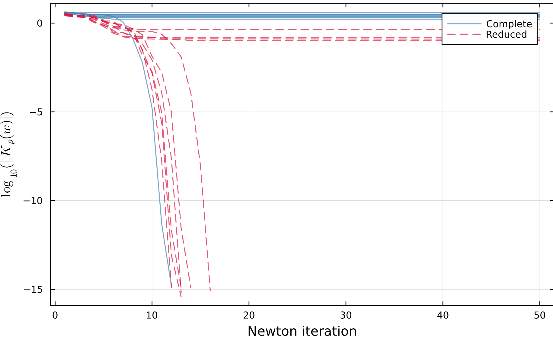
Fixed problem, random init ( \rho=0.01 , K=2 , 10 runs)
