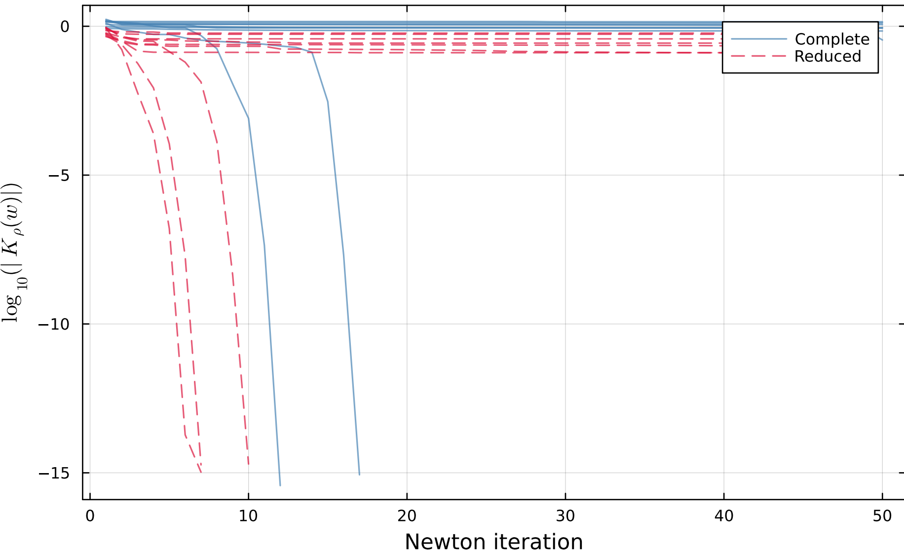
Random problems, canonical init ( \rho=0.001 , K=4 , 10 problems)
