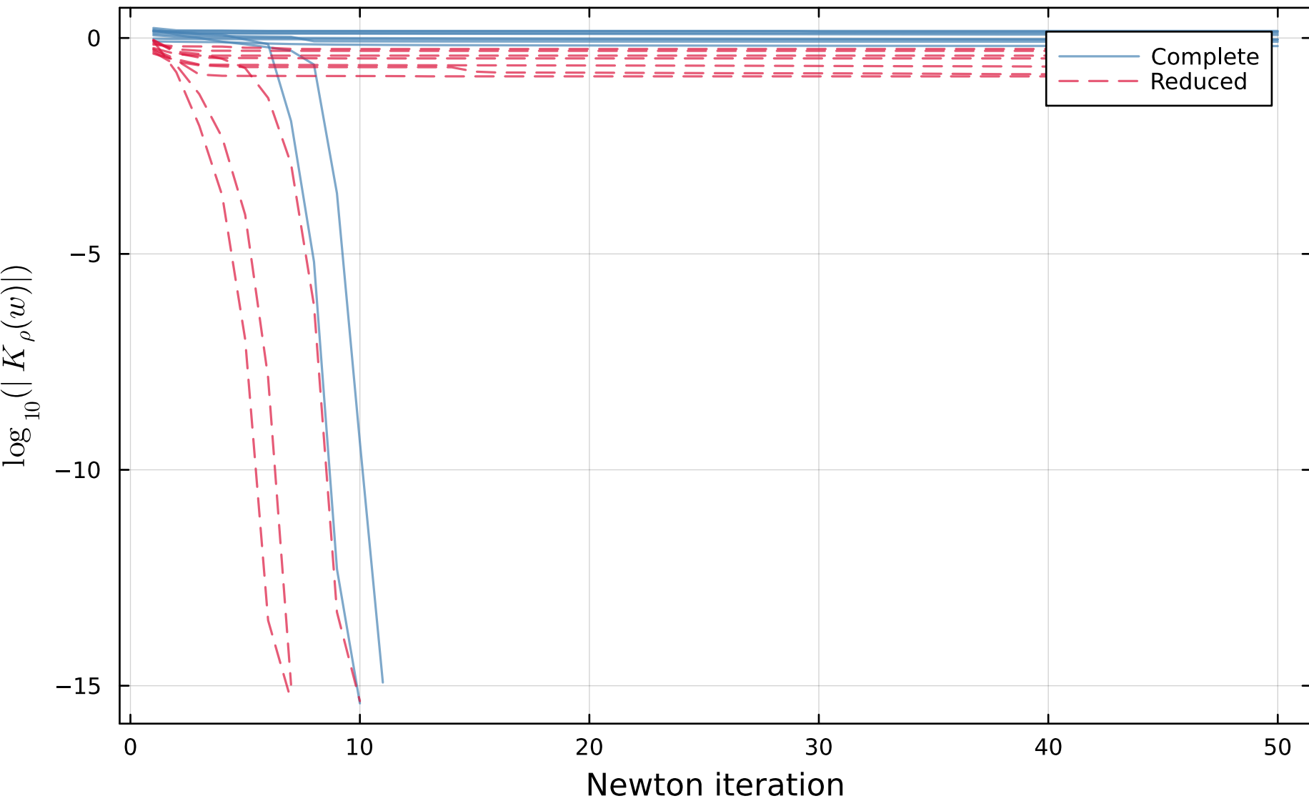
Random problems, canonical init ( \rho=0.01 , K=4 , 10 problems)
