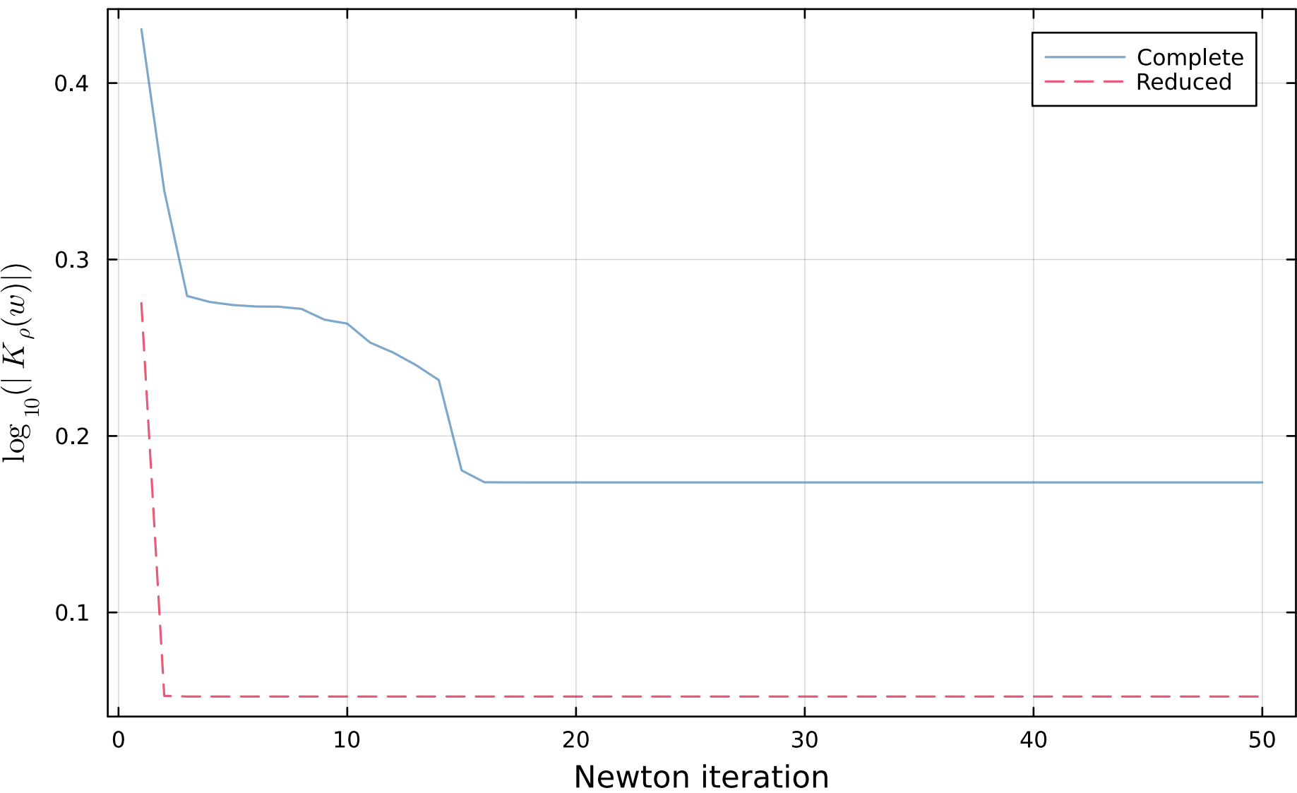
Random QP problems, canonical init ( \rho=1.0 , K=2 , 1 problems)
