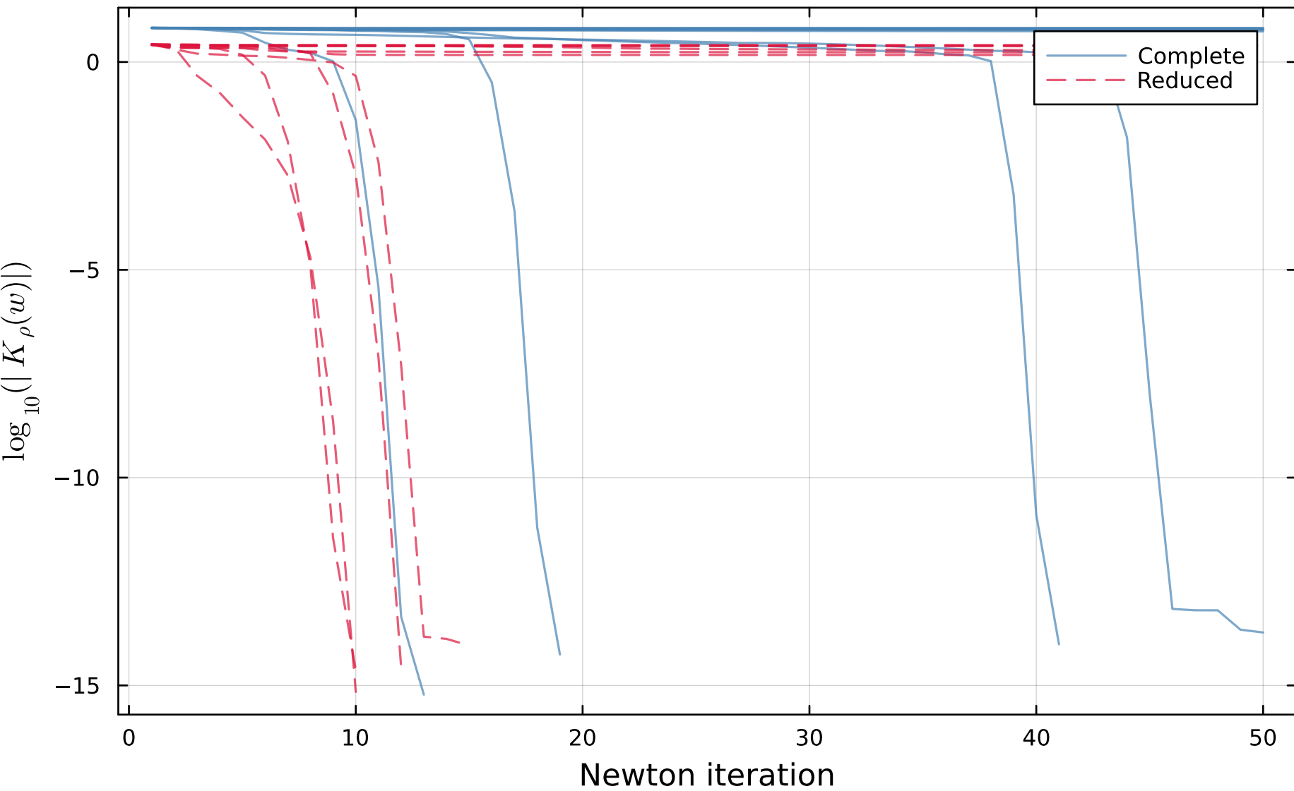
Random problems, canonical init ( \rho=1.0 , K=4 , 10 problems)
