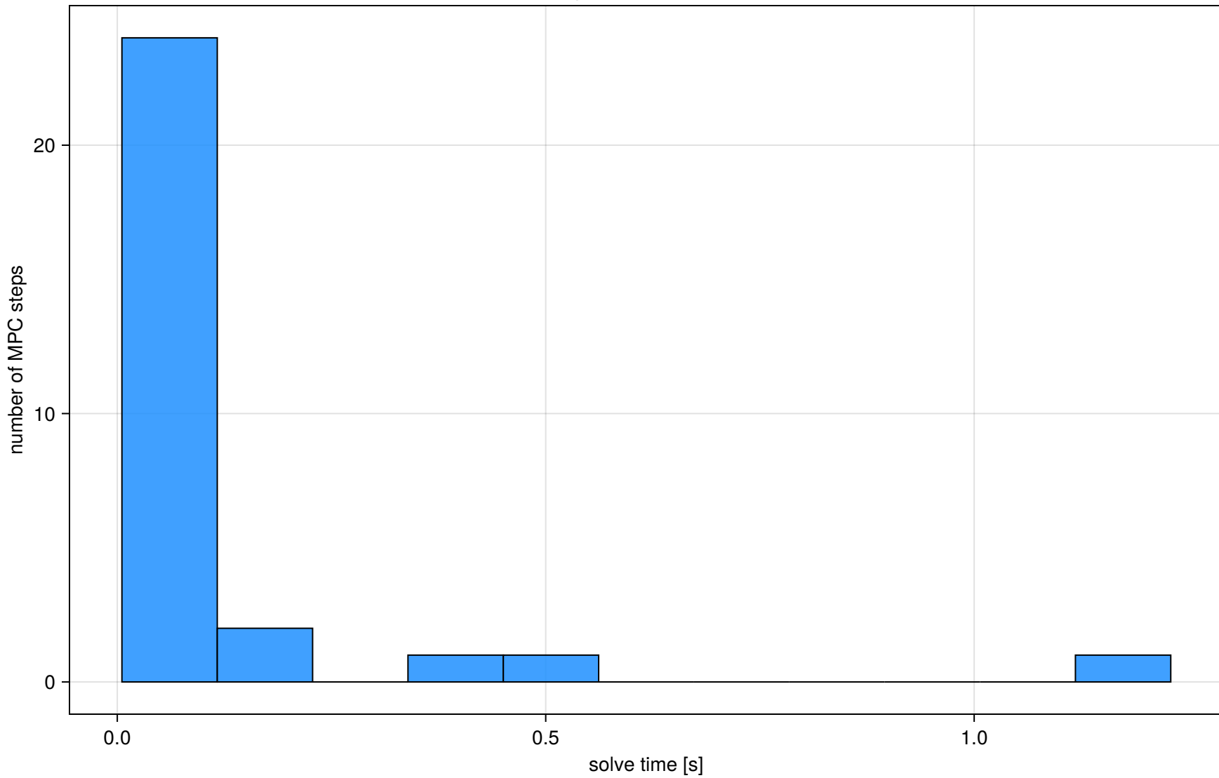
Warm-solve times (step 1 excluded: 62.5 s incl. one-time JIT)
