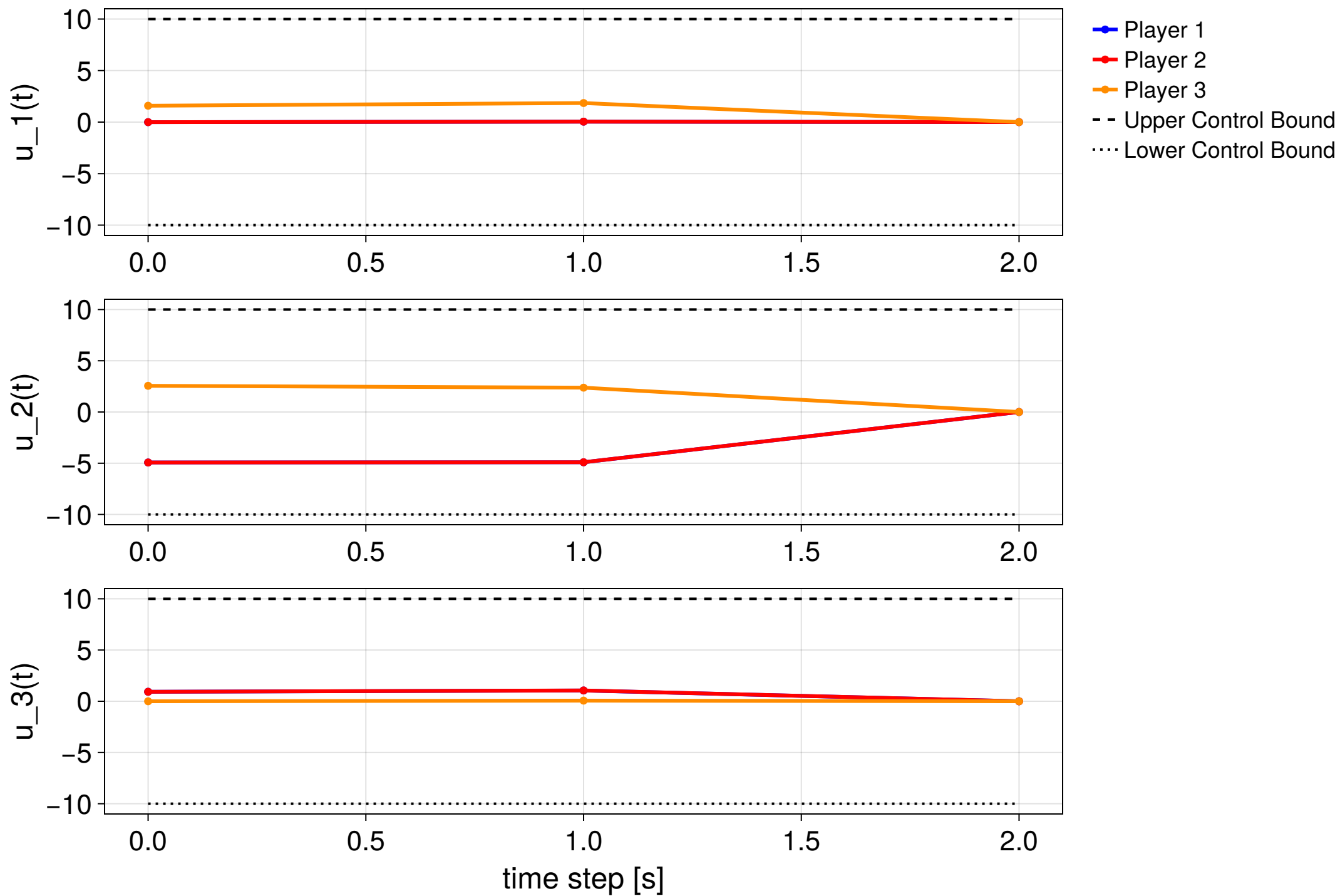
Closed-loop receding-horizon execution (2 steps) — non-converged steps: 2
