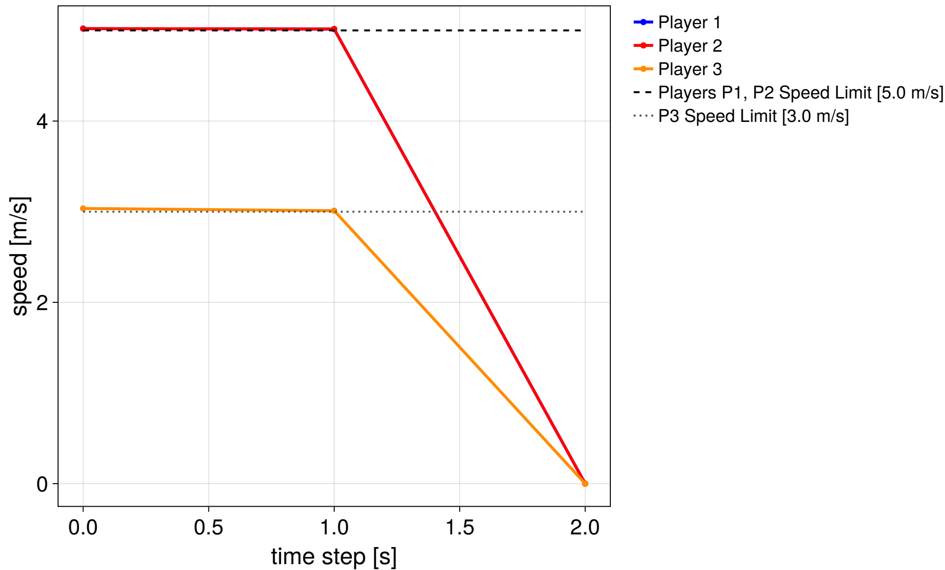
Closed-loop receding-horizon execution (2 steps) — non-converged steps: 1, 2
