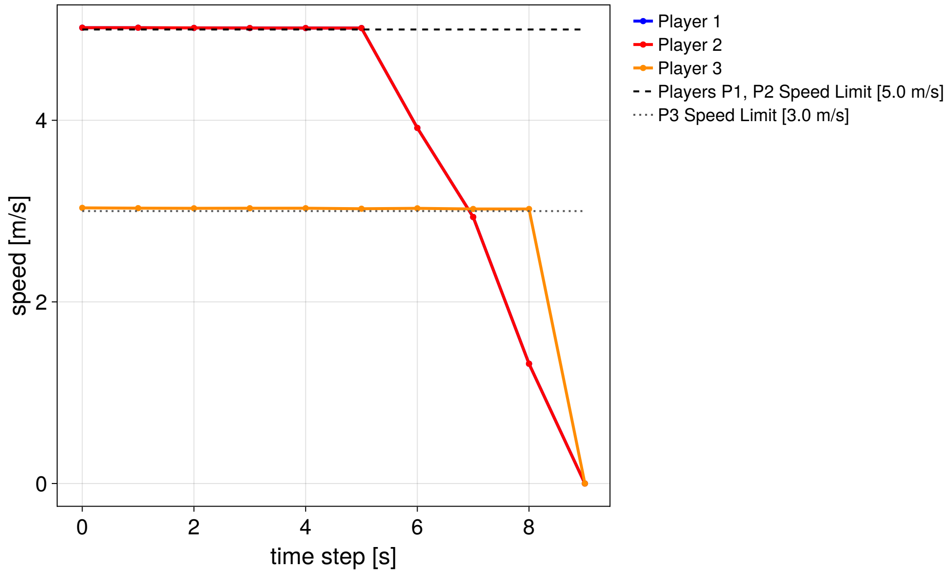
MPC step 1/2 — NOT CONVERGED (KKT error 1.4)
