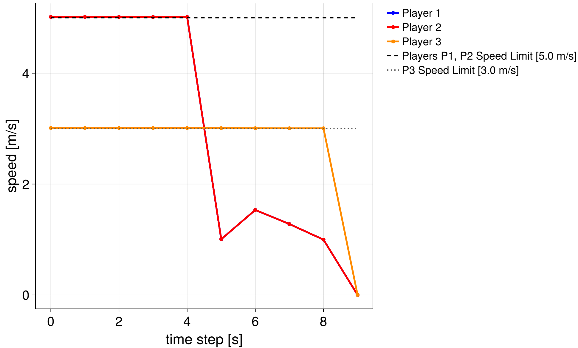
MPC step 2/2 — NOT CONVERGED (KKT error 0.135)
