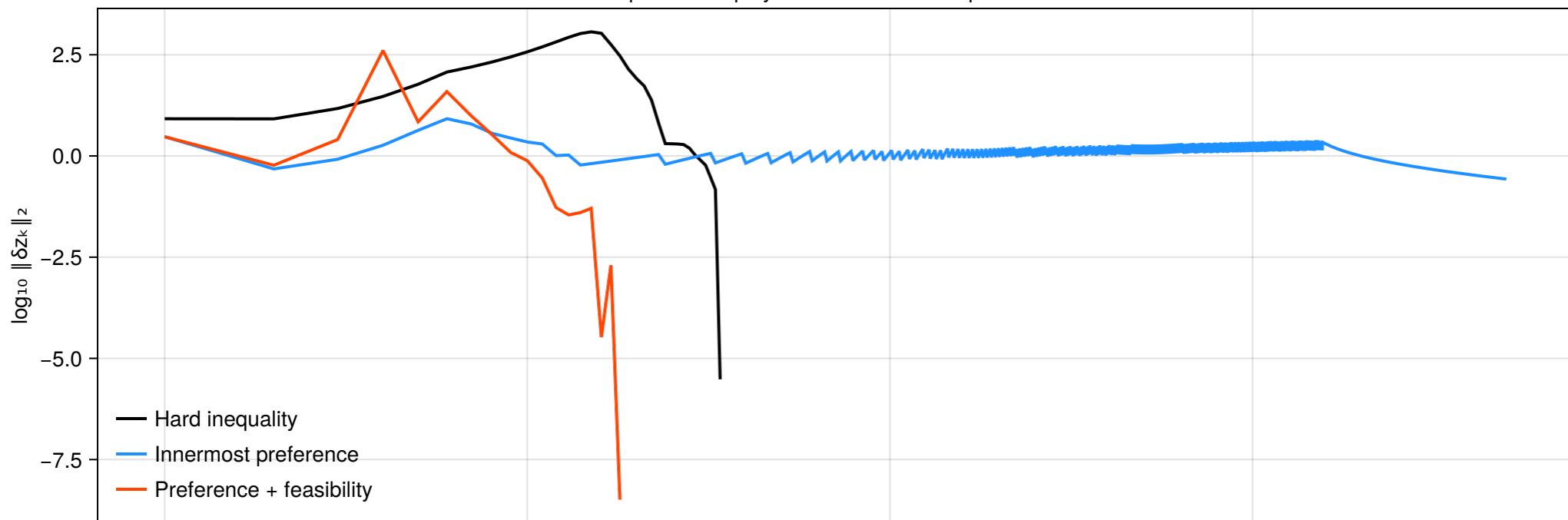
Explicit three-player solve: Newton step histories
