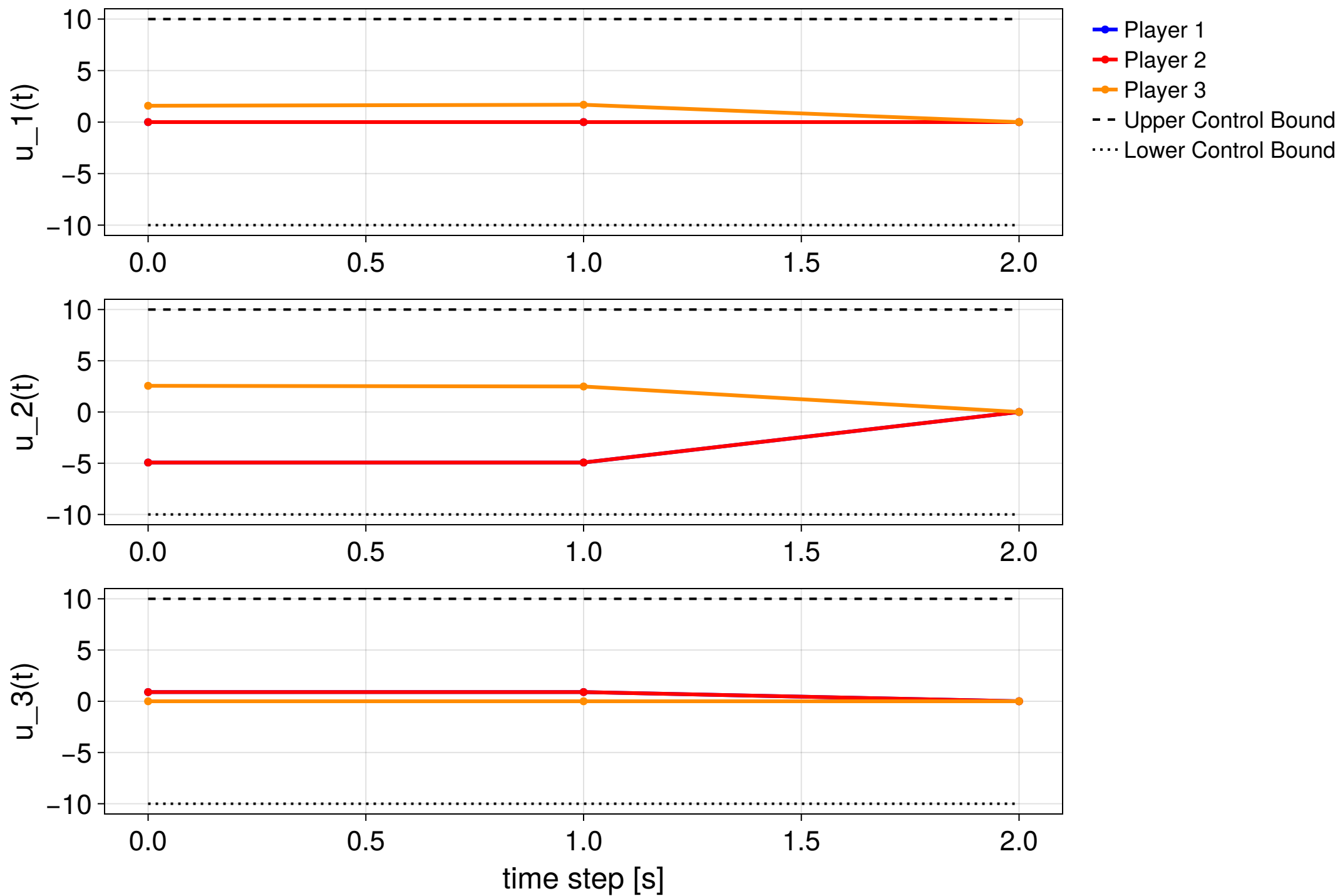
Closed-loop receding-horizon execution (2 steps)
