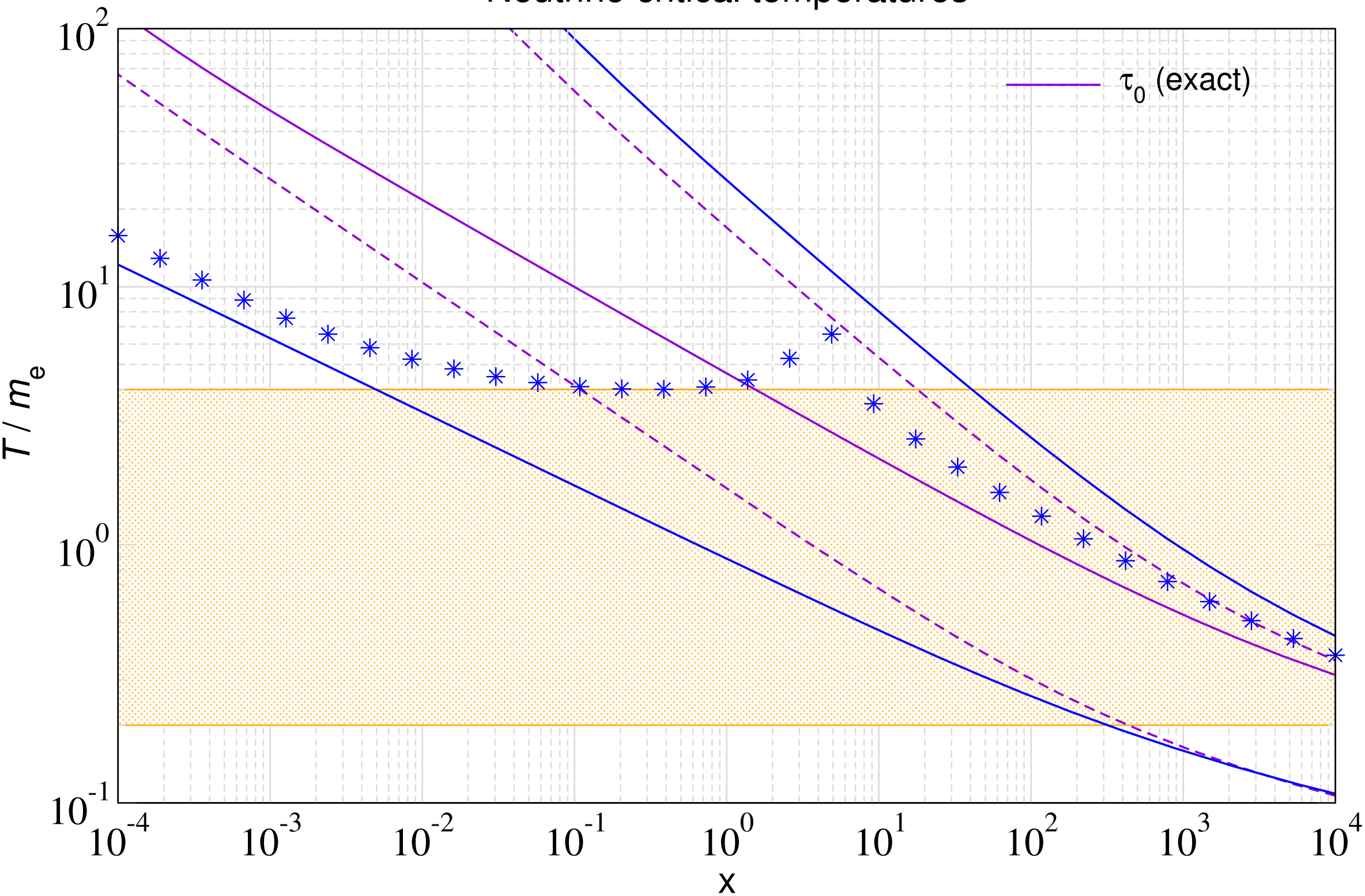
Neutrino critical temperatures
