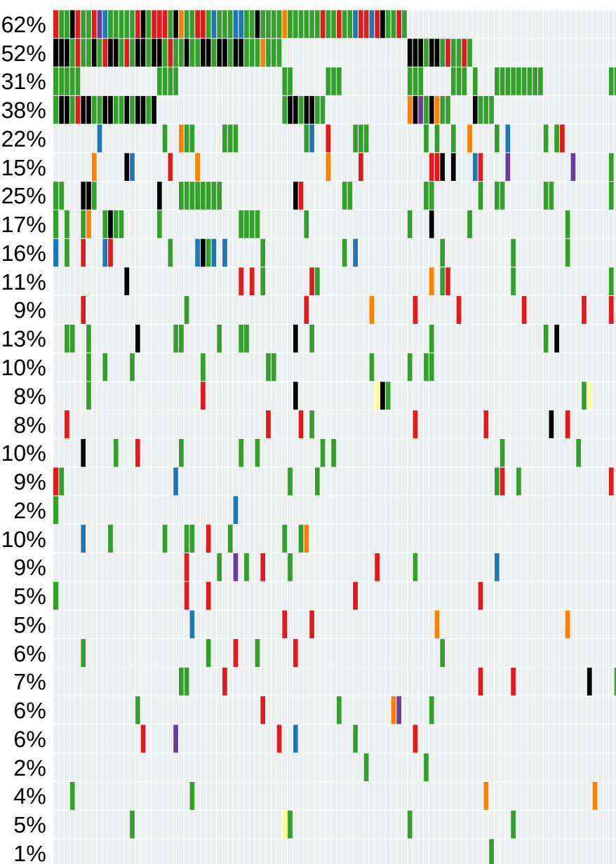
LUAD-LOY (N = 104)
