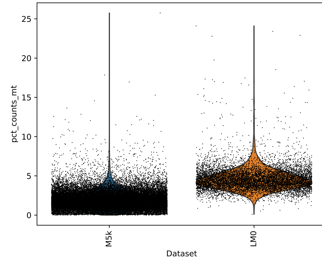
Pct Counts Mt
