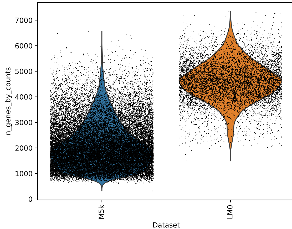
N Genes By Counts
