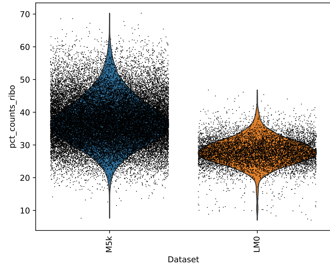
Pct Counts Ribo
