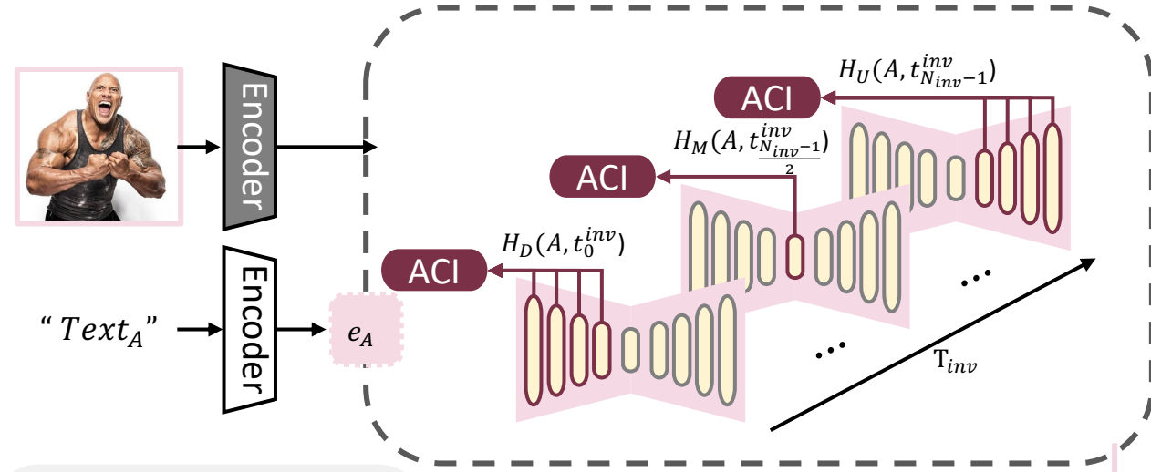
(a) DDIM Inversion (Total Iteration = N_{inv} )
