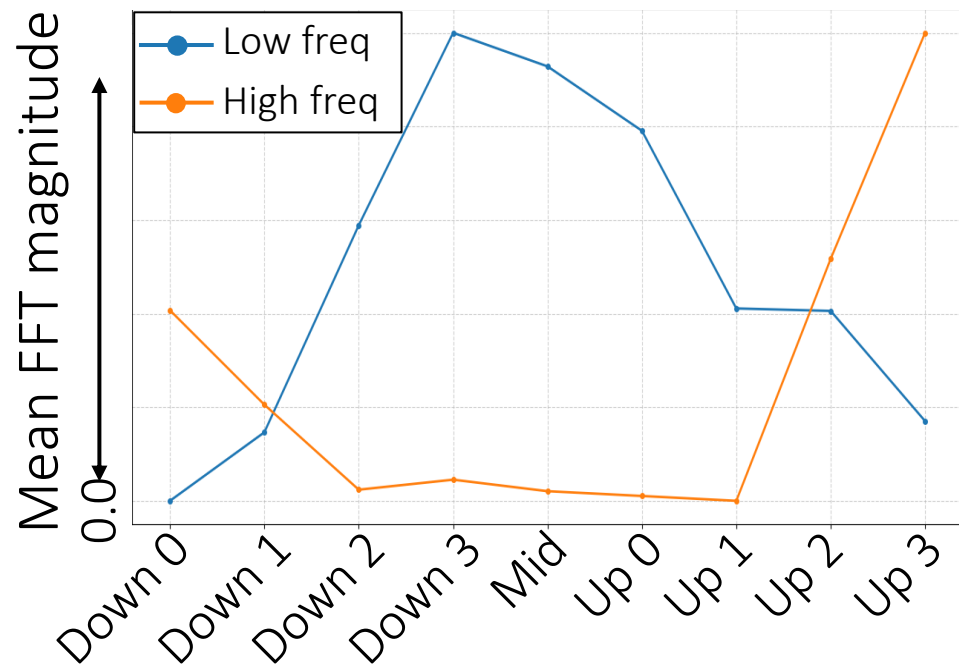
(a) Frequency component on DDIM inversion feature
