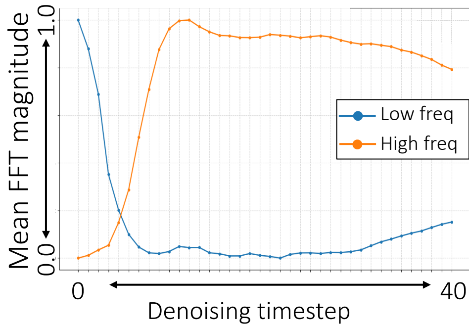
(b) Frequency component on diffusion timestep
