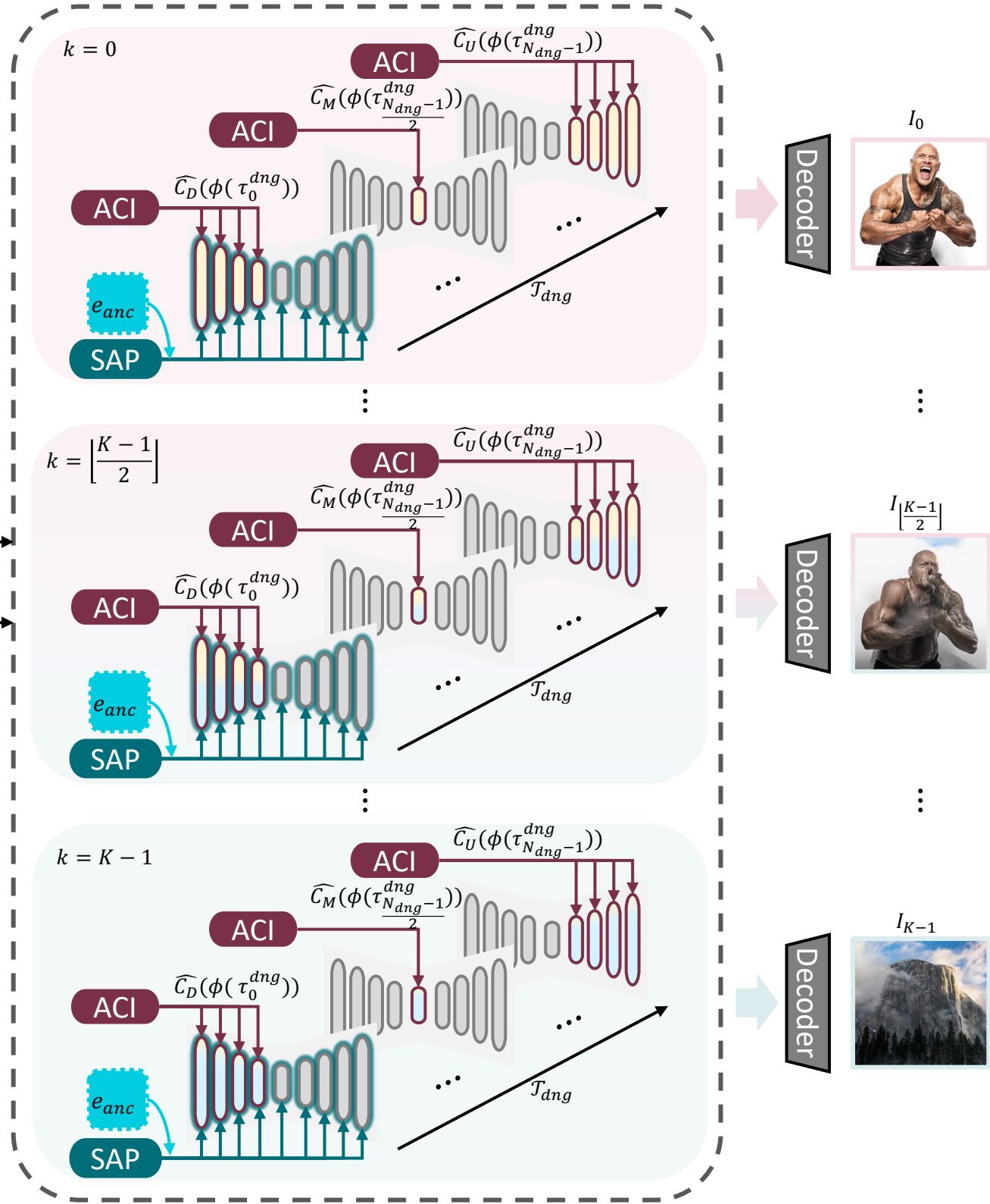
(b) Denoising Process (Total Iteration = N_{dng} )
