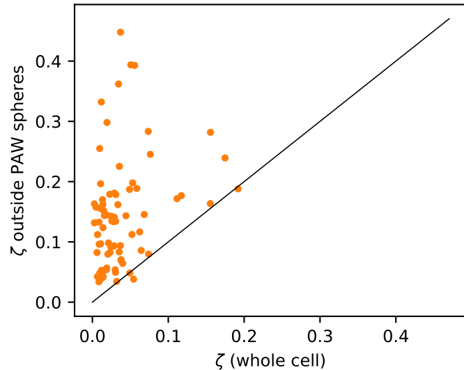
(b) Spearman 0.34
