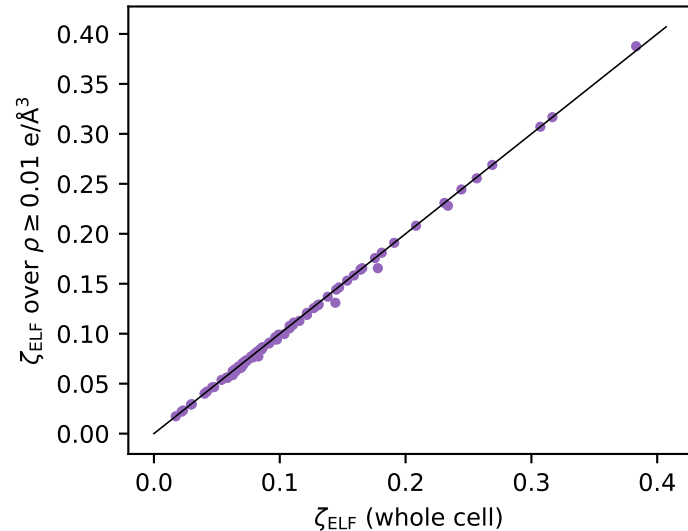
(c) Spearman 1.00
