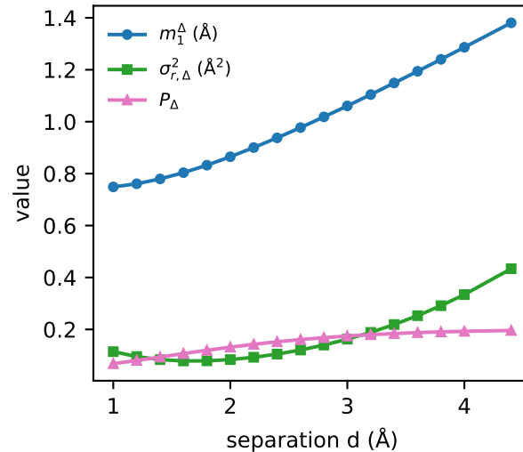
(c) moments and polarity vs bond length
