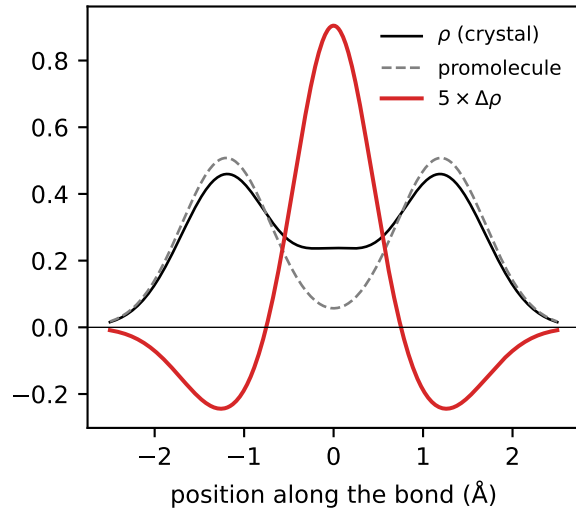
(a) bond-charge model, d = 2.4 \text{ \AA} , q = 0.2
