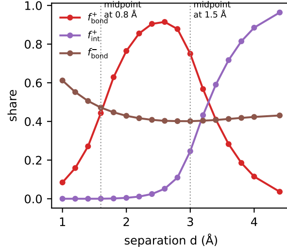
(b) shell shares vs bond length ( q = 0.2 )
