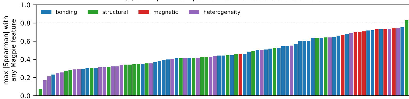
(e) overlap with composition: 86 of 87 descriptors below 0.8
