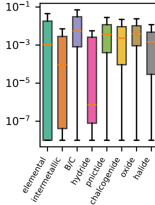
(e) overlap with composition: 86 of 87 descriptors below 0.8
