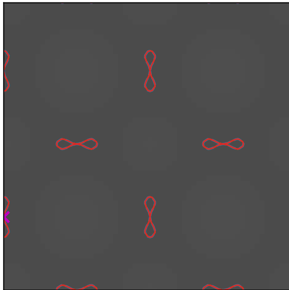
Al (fcc metal) (ab plane; levels a/b/c = 0.203/0.203/0.203)
