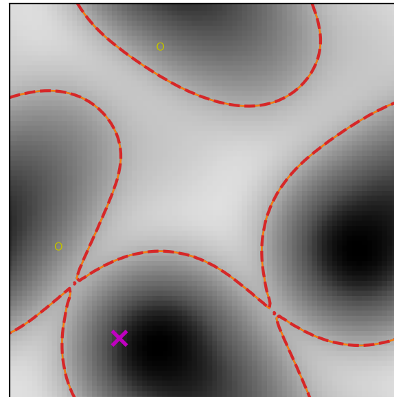
CO2 (molecular solid) (ca plane; levels a/b/c = 0.043/0.043/0.043)
