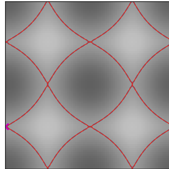
NaCl (ionic) (ab plane; levels a/b/c = 0.029/0.029/0.029)
