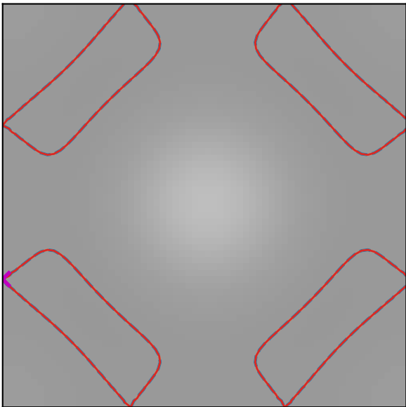
Na (bcc, free-electron metal) (ab plane; levels a/b/c = 0.030/0.030/0.030)
