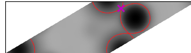
Ca2N (layered electride) (ab plane; levels a/b/c = 0.260/0.260/0.260)
