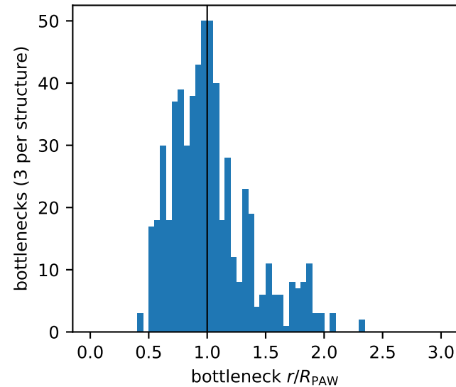
(a) bottlenecks vs PAW spheres (200 structures)
