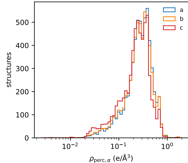
(a) percolation levels
