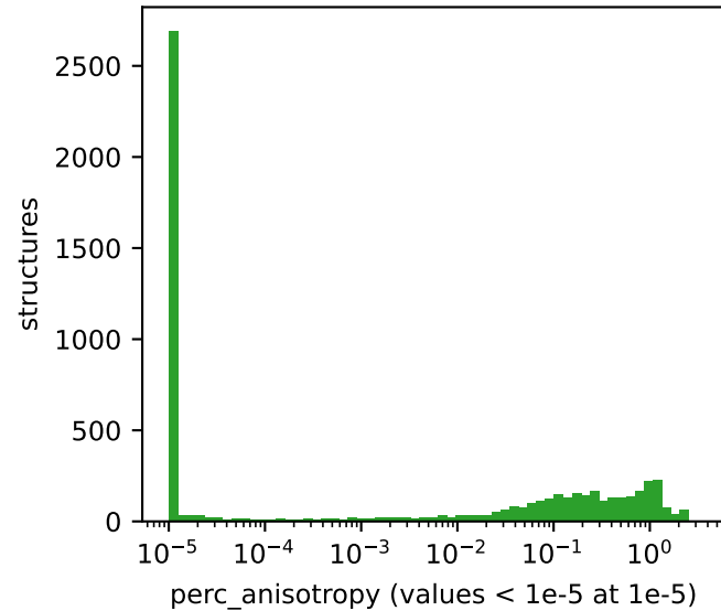
(b) perc_anisotropy
