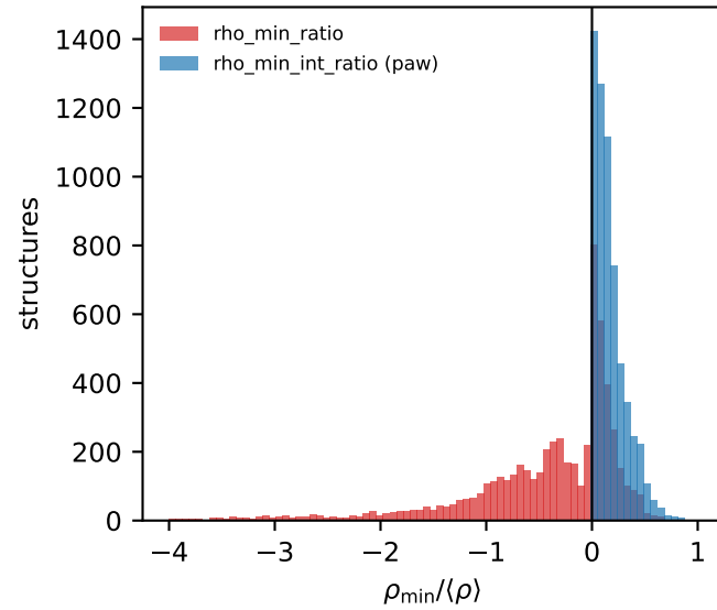
(c) density floor
