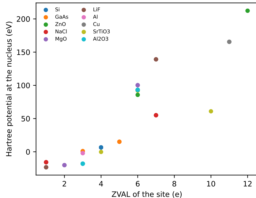
(a) site potentials follow the valence count
