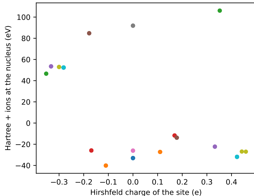
(b) full electrostatic site potential
