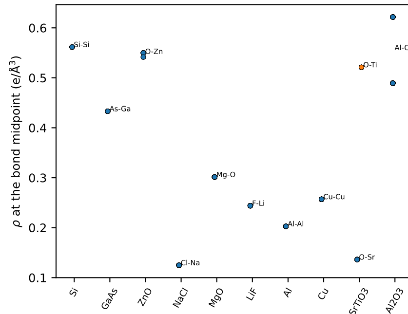
(c) midpoint densities of the census bonds
