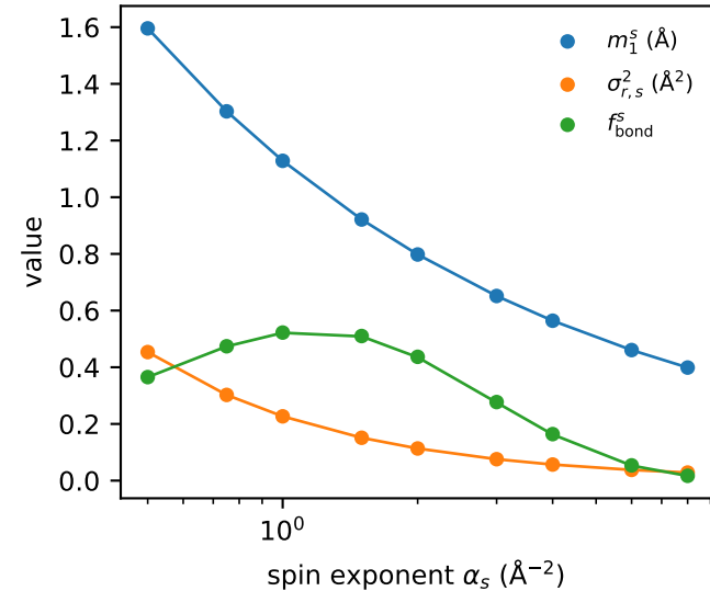
(a) one magnetic atom: lines exact
