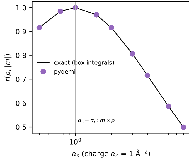
(b) spin-charge correlation
