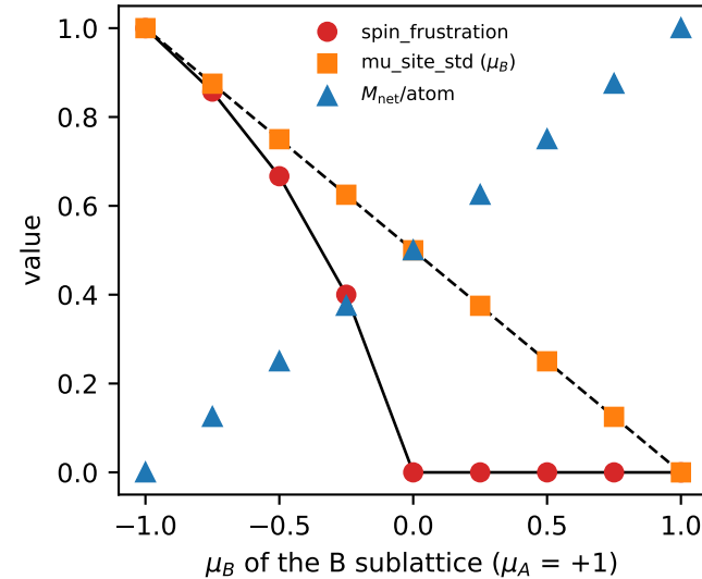
(c) two sublattices: FM \rightarrow ferri \rightarrow AFM
