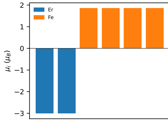
ErFe2 (Laves, ferrimagnet): std 2.29 \mu_B , F_s 0.894
