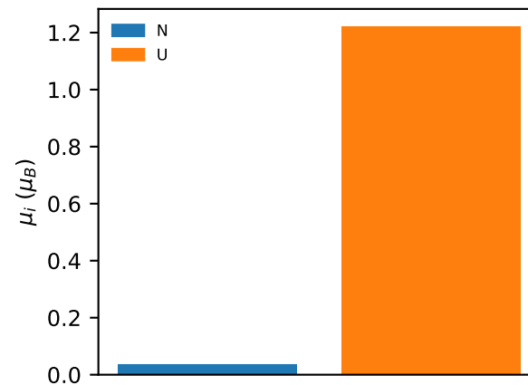
UN (5f): std 0.59 \mu_B , F_s 0.000
