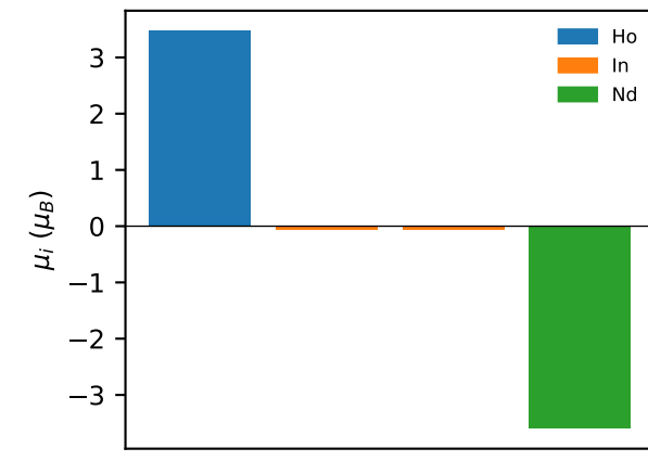
NdHoIn2 (compensated 4f): std 2.50 \mu_B , F_s 0.962
