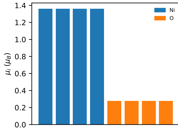
NiO (FM cell): std 0.54 \mu_B , F_s 0.000
