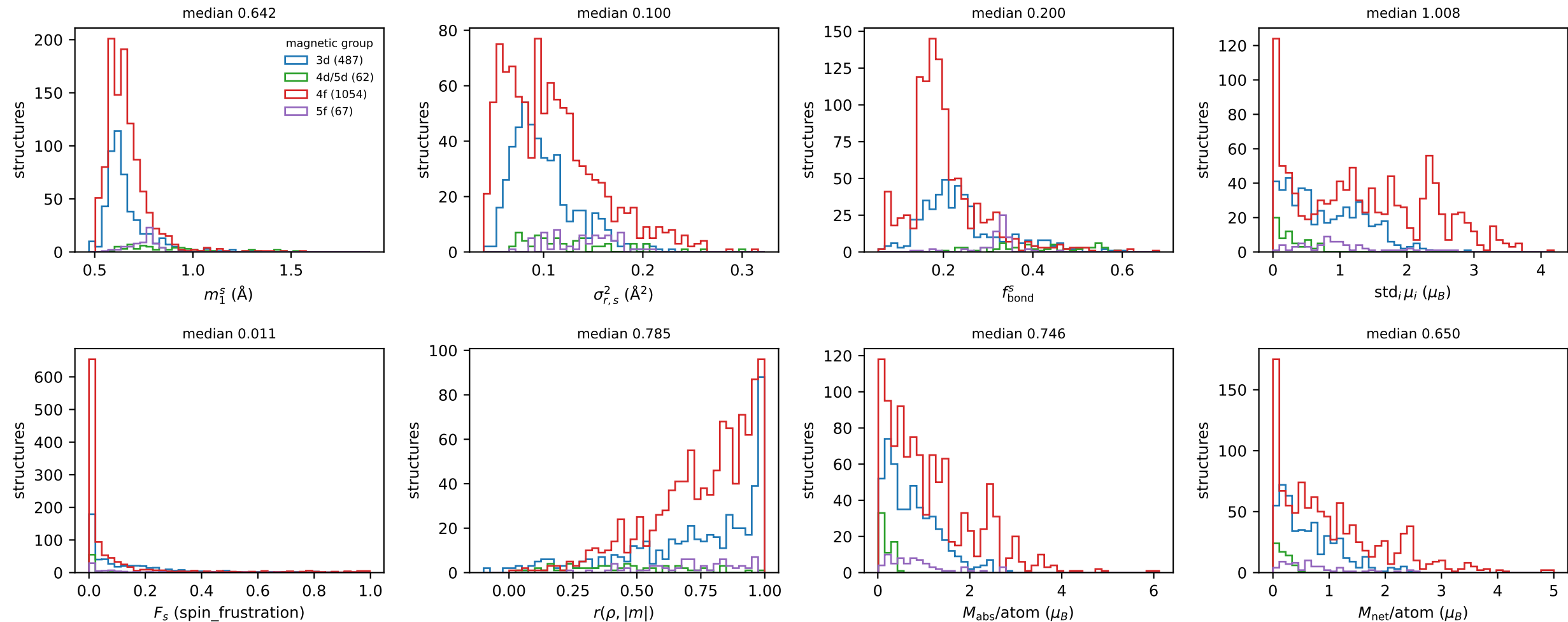
Distributions over the 1,679 magnetic structures (of 6,059), by magnetic-element group
