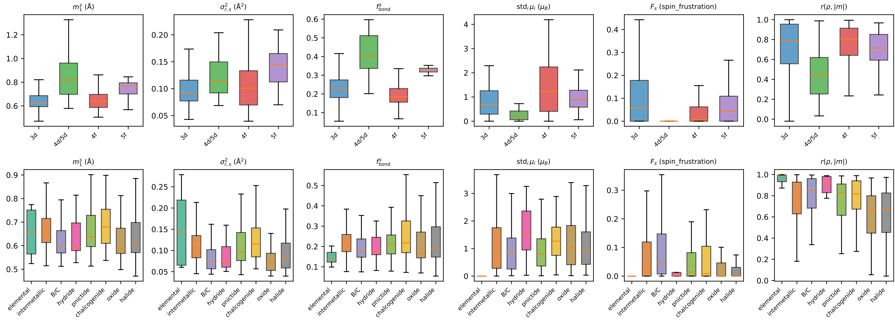
Magnetic structures by magnetic-element group (top) and chemical class (bottom; classes with \geq 5 magnetic structures)
