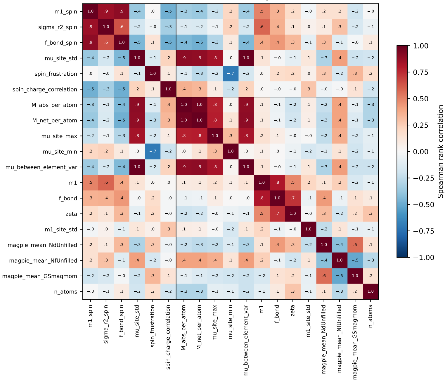
Rank correlations over the 1,679 magnetic structures
