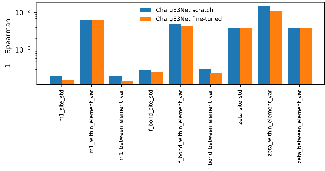
(b) rank agreement across the test structures
