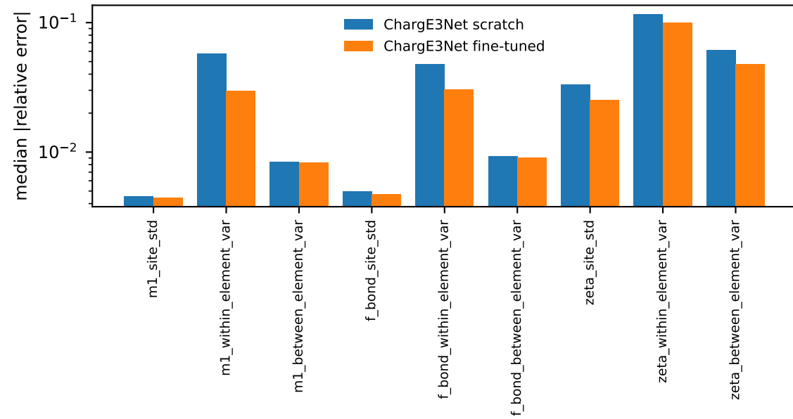
(a) descriptor from predicted vs DFT density
