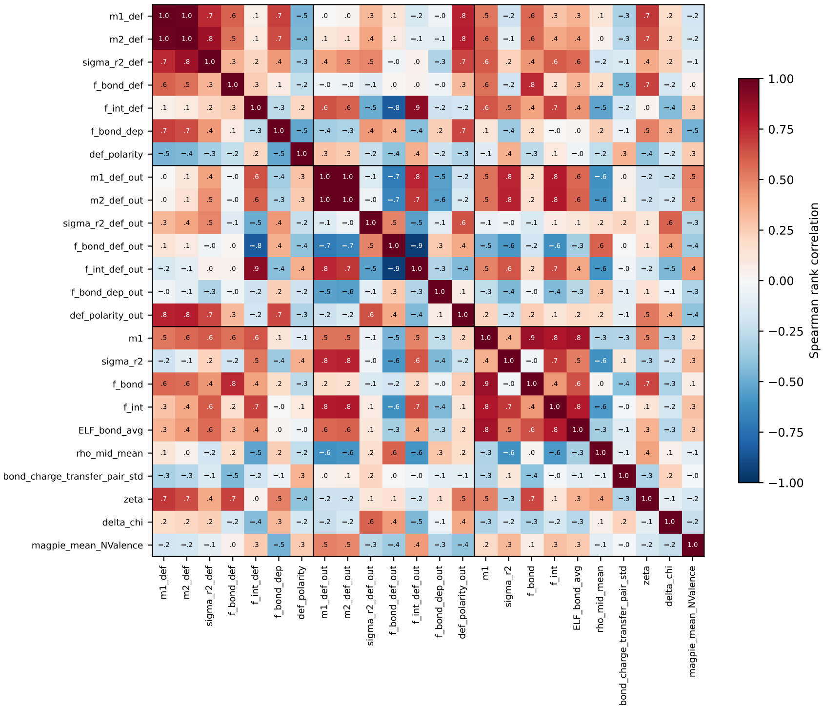
Rank correlations over the 6,059 structures
