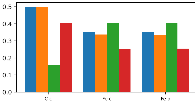
Ba2SnO4 (Ruddlesden-Popper): per-site f_{\text{bond}}
