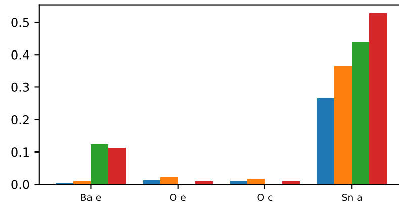
Ba2SnO4 (Ruddlesden-Popper): per-site \zeta
